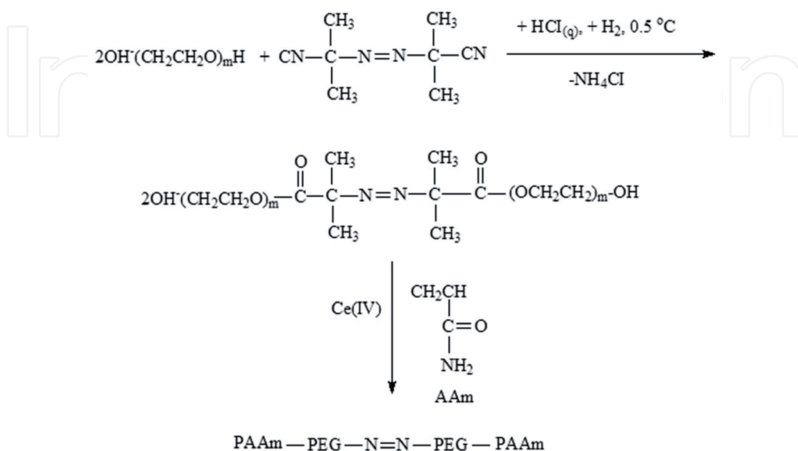
Figure 3. Polymerization of acrylamide with poly(ethylene glycol)azoester/Ce 4+ redox system.
