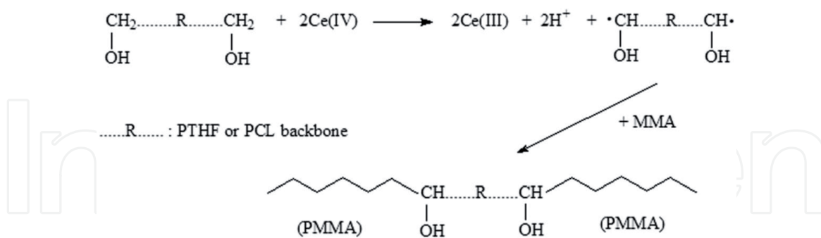
Figure 1. Synthesis of PMMA-b-PCL-b-PMMA block copolymer with PCL-diol/Ce(IV) redox systems.
