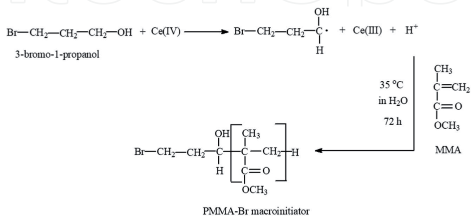
Figure 8. Figure 1 Chemical synthesis of PMMA-Br macroinitiator via redox polymerization.
