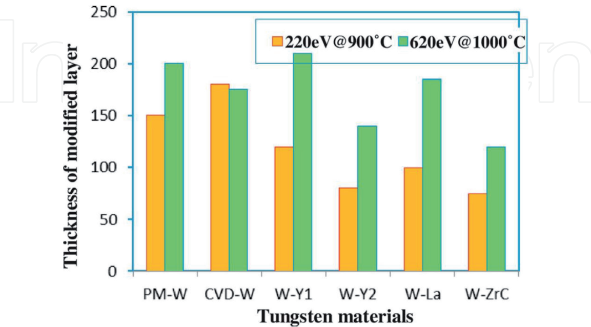
Figure 5. Thickness of modified layers in various tungsten materials under the He + irradiation of 220 eV at 900°C and 620 eV at 1000°C [58].
