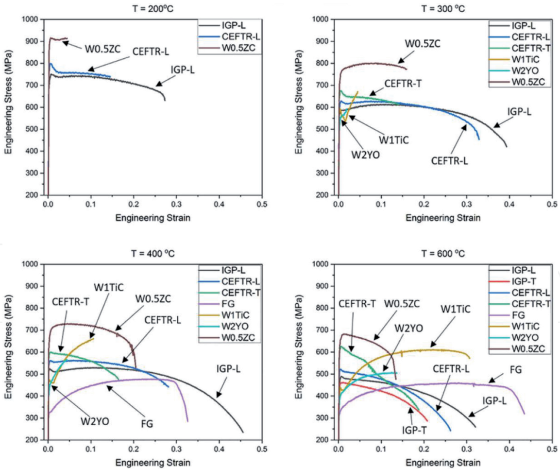
Figure 2. The tensile stress of various W materials [51].
