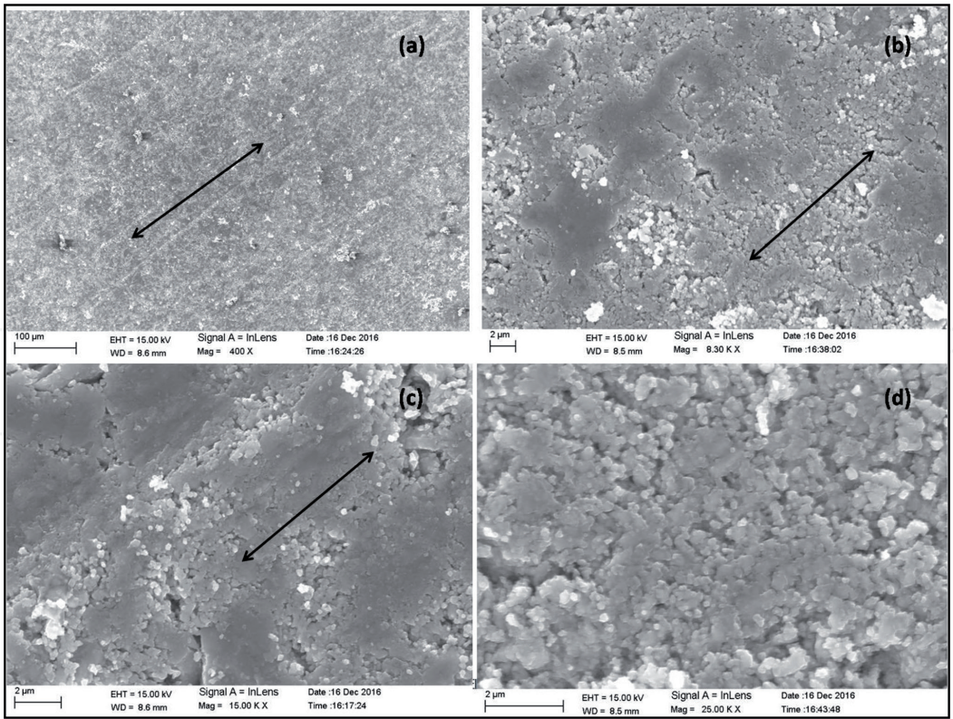
Figure 8. SEM images of unclean polished white PCD sample at successive higher magnifications.
