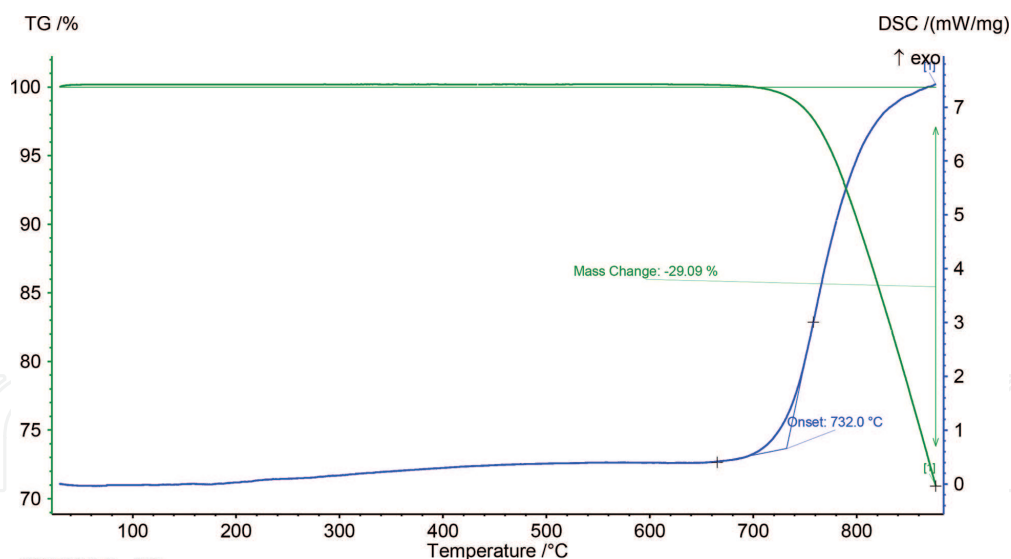
Figure 3. TGA and DSC curves for heating CVD diamond in air.
