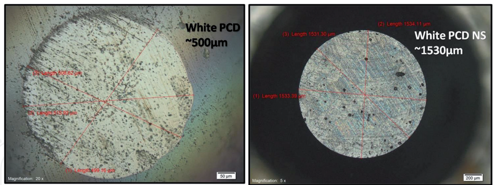
Figure 12. Wear scar diameters on counterbody \text{Si}_3\text{N}_4 ball against white PCD (a) polished surface and (b) nucleation side surface.
