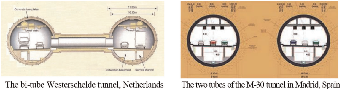
Figure 3. Common layouts of road tunnels.
