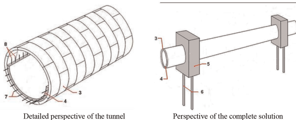
Figure 4. Illustration of the TISB concept.
