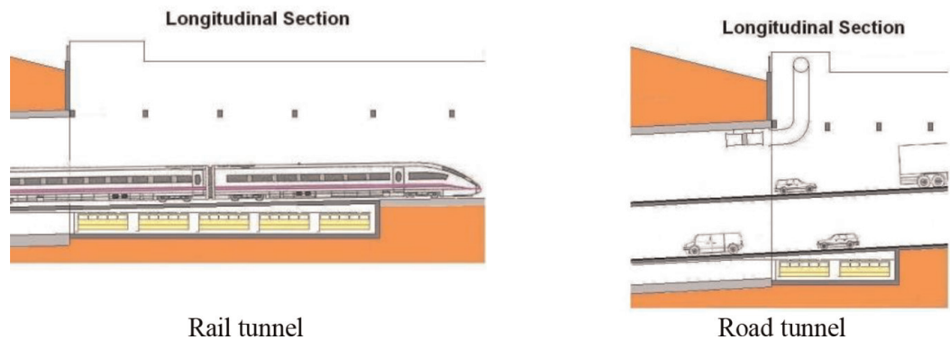
Figure 19. Optimized TBM tunnel alternative. Portals of the tunnels.
