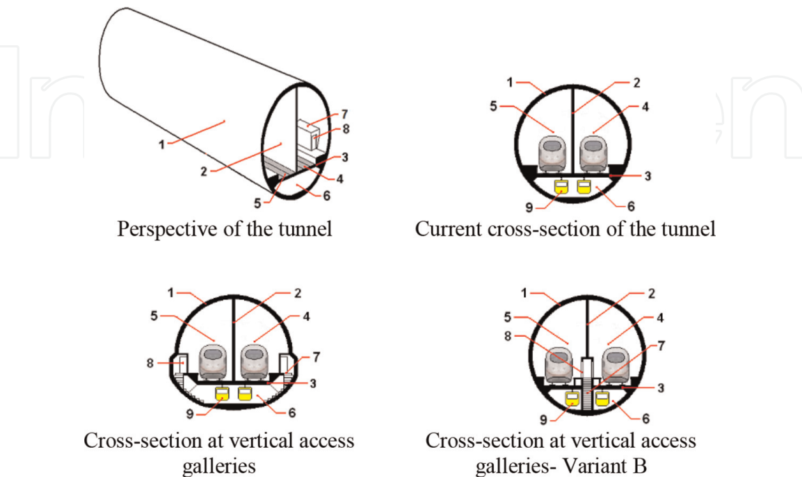
Figure 5. Illustration of the TMG concept.
