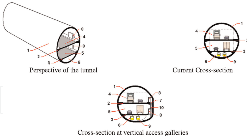
Figure 6. Illustration of the TMF concept.
