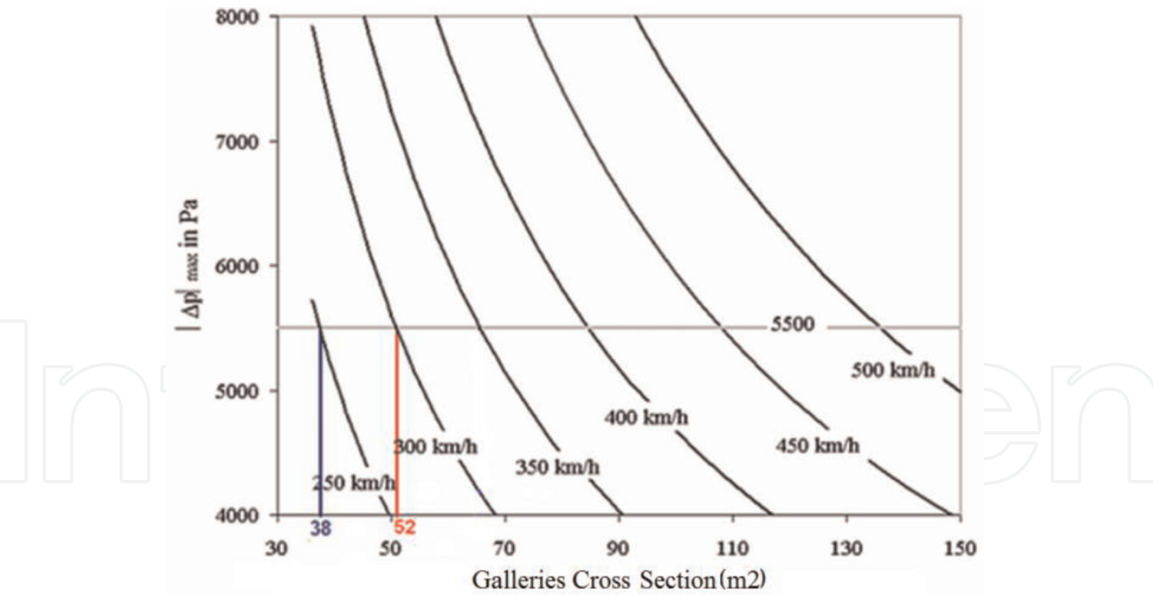
Figure 7. Relationships between the cross-section of the rail galleries of the tunnels and the speed of the trains.
