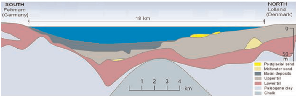
Figure 14. Geotechnical conditions of the site.
