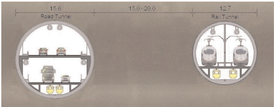
Figure 16. Optimized TBM tunnel alternative. Current cross-section.
