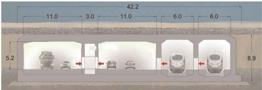
Figure 15. Immersed tunnel solution. Current cross-section.
