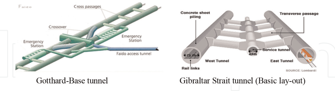
Figure 2. Common layouts of rail tunnels.
