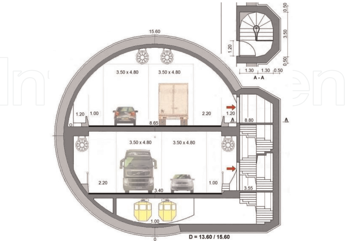
Figure 12. Proposed TBM tunnel solution for the Algés-Trafaria crossing. Cross-section at vertical access galleries.
