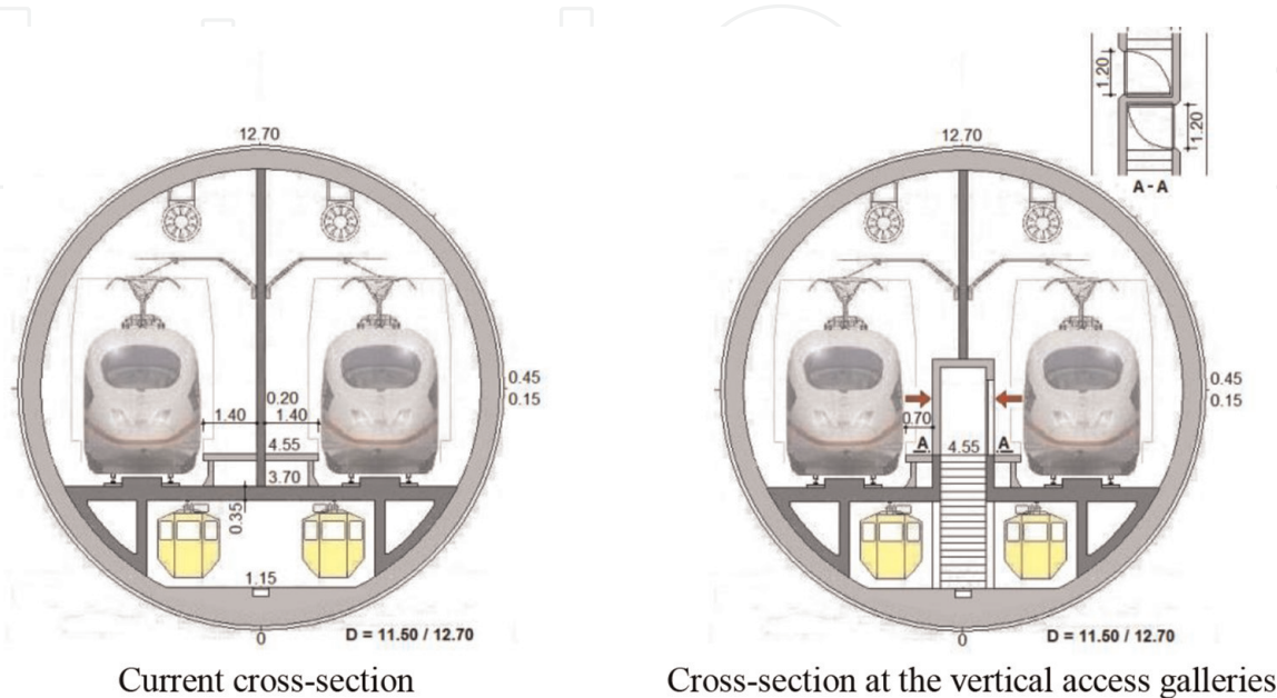
Figure 17. Optimized TBM tunnel alternative. Cross-section of the railway tunnel.
