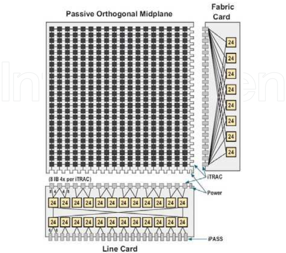
Fig. 2. DS3456 Internal Connectivity
