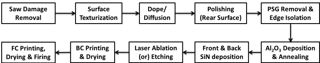
Figure 3. PERC process flow.
