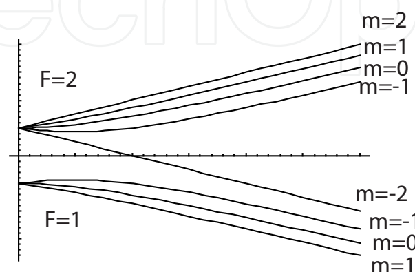
Fig. 1. Dependence of Zeeman sublevels on magnetic field for the case of I=3/2 .
