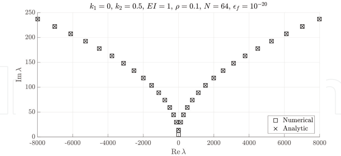
Figure 1. Graphical representation of the eigenvalues of the discrete and “continuous” operators ( \mathcal{K} > 1 ).
