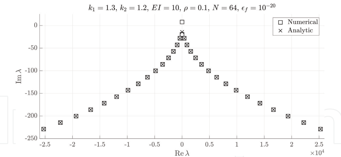
Figure 2. Graphical representation of the eigenvalues of the discrete and “continuous” operators ( K < -1 ).
