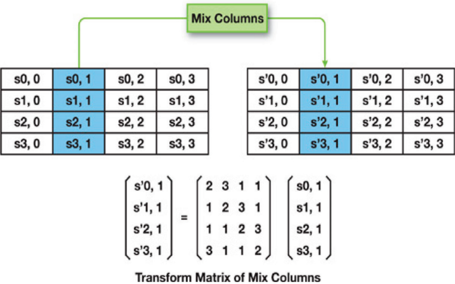
Figure 5. Mix column stage.
