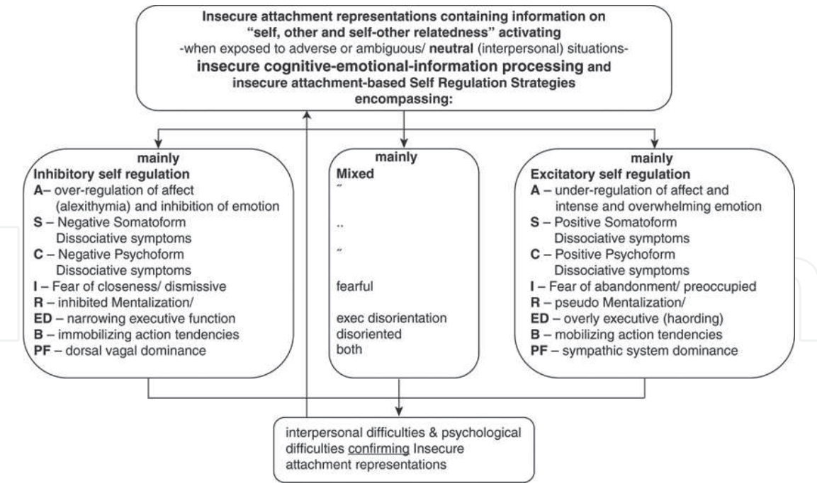
Figure 1. Three qualitatively different self-regulation styles or different networks: inhibitory, excitatory, and combined inhibitory and excitatory (IE) regulation operating in self-sustaining, vicious cycles due to the presence of hysteresis in strongly connected childhood trauma-related symptom networks.
