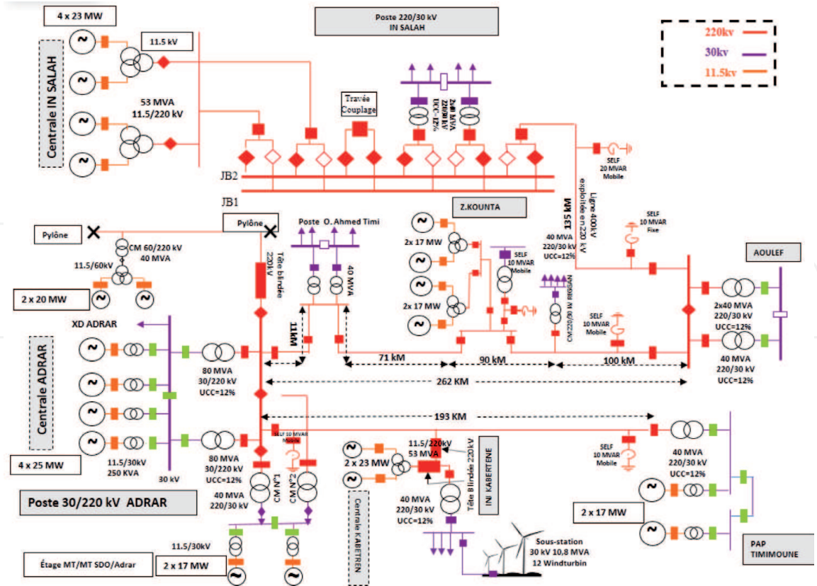
Figure 7. Adrar grid.
