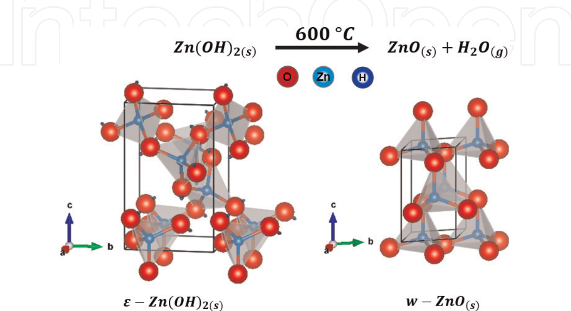
Figure 3. (a) Unitary cell of \epsilon\text{-Zn(OH)}_2 , (b) representation of polyhedra of the unitary cell of the wulfingite, (c) unitary cell of \text{ZnO} , and (d) representation of polyhedra of the unit cell of the wurtzite.
