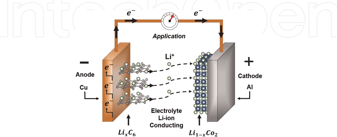
Figure 1. Schematic of a Li-ion cell.
