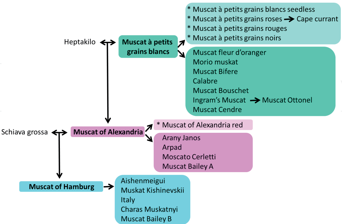
Figure 2. Genetic relationships among Muscat varieties. Muscat à petits grains blancs is the progenitor of ancient variety Muscat of Alexandria and the putative ancestor of all the Muscat varieties. From them, additional Muscat varieties are derived by spontaneous or directed hybridizations (see [55] and Vitis International Variety Catalog ( http://www.vivc.de )) as well as through somatic variation (*).
