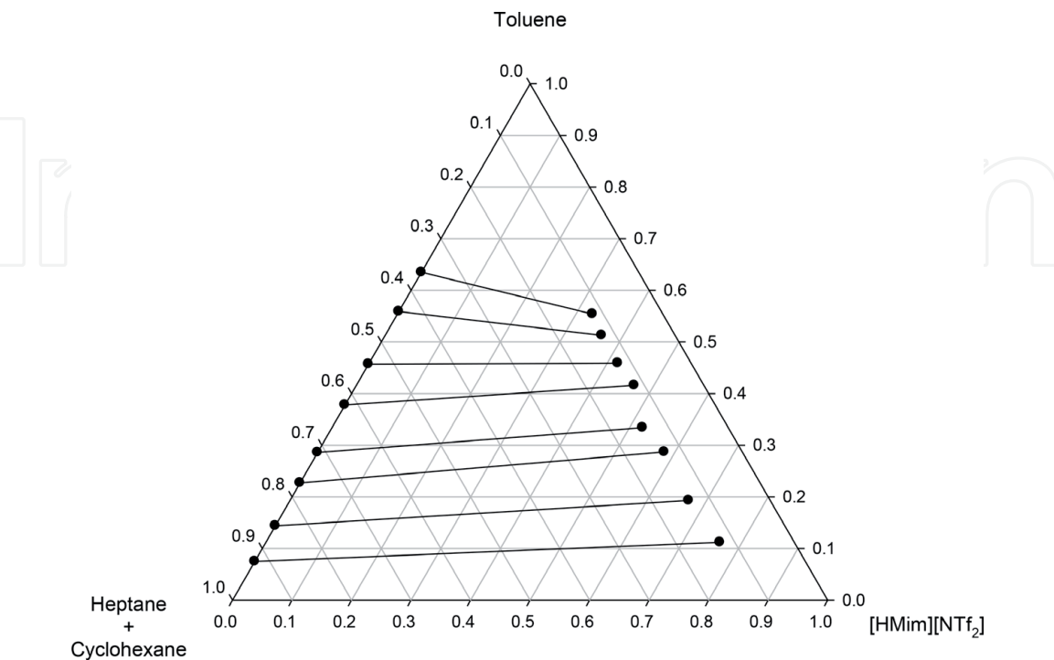
Figure 3. Tie lines for the quaternary systems heptane + cyclohexane + toluene + [HMim][NTf 2 ].
