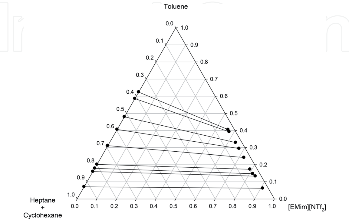
Figure 2. Tie lines for the quaternary systems heptane + cyclohexane + toluene + [EMim][NTf 2 ].
