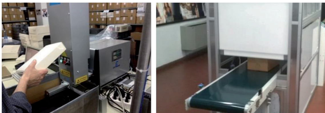
Figure 3. RFId reading post, Box label printing and application. Source: Oscalito.
