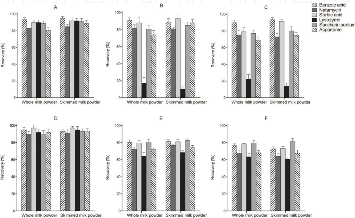
Figure 2. Recovery results of the six different sample preparation methods. The left group in A–F represents the whole milk powder matrix, and the right group in A–F represents the skimmed milk powder matrix. The six food additives: benzoic acid, sorbic acid, natamycin, lysozyme, aspartame, and saccharin sodium. (A) Method A (liquid-liquid extraction). (B) Method B (precipitation based on sodium tungstate). (C) Method C (precipitation based on potassium ferrocyanide). (D–F) Method D–F (solid phase extraction): (D) Poly-Sery HLB SPE, (E) CNWBOND LC-C18 SPE, and (F) Poly-Sery MAX SPE.
