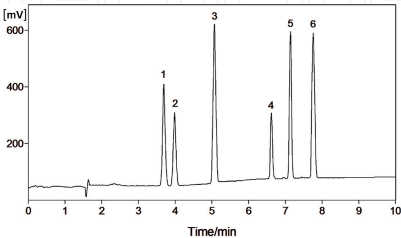
Figure 3. Chromatogram of mixed standard solutions. (1) Benzoic acid, (2) sorbic acid, (3) saccharin sodium, (4) natamycin, (5) aspartame, and (6) lysozyme.
