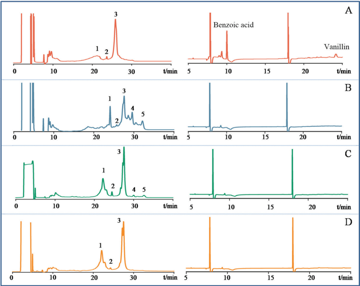
Figure 9. Chromatograms of four brands of commercial milk and milk powders. (A) Infant formula milk powder 1, (B) infant formula milk powder 2, (C) skimmed milk powder, and (D) bovine milk. (1) \alpha -Casein ( \alpha -CN), (2) \alpha -lactalbumin ( \alpha -Lac), (3) \beta -casein ( \beta -CN), (4) \beta -lactoglobulin B ( \beta -LgB), and (5) \beta -lactoglobulin A ( \beta -LgA).
