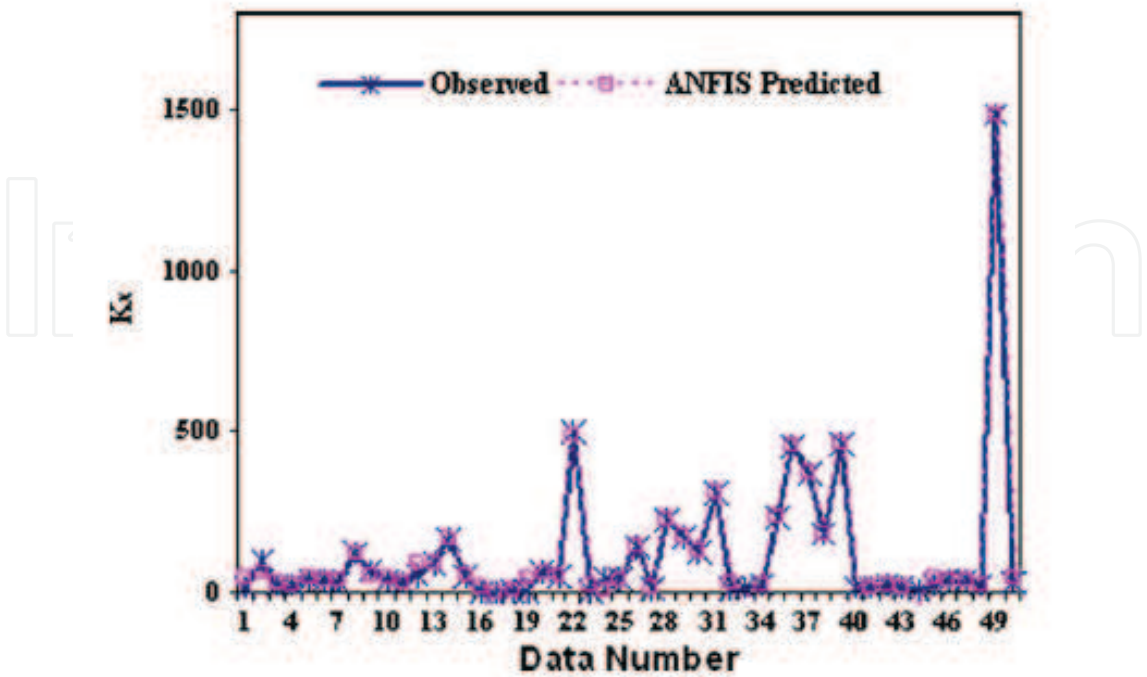
Fig. 4. Performance of ANFIS model results in training step
