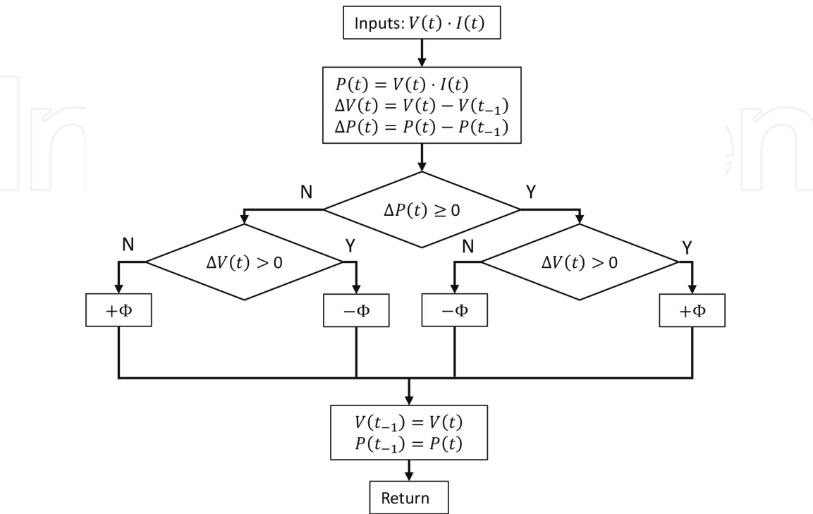
Figure 19. P&O algorithm flowchart.
