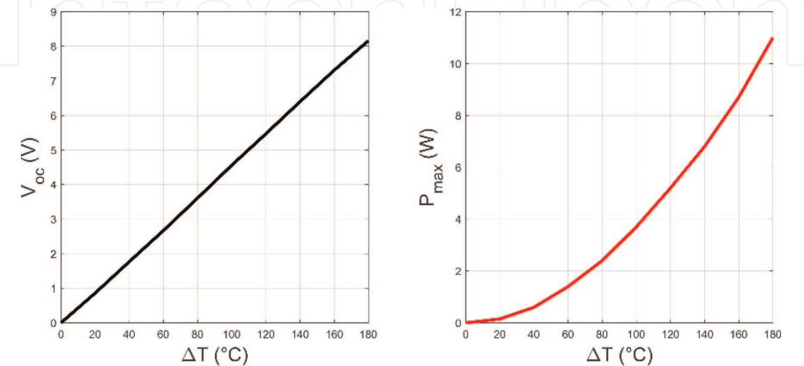
Figure 4. TEG cell characteristics as a function of delta temperature; on the left the open-circuit voltage and on the right the available maximum power.
