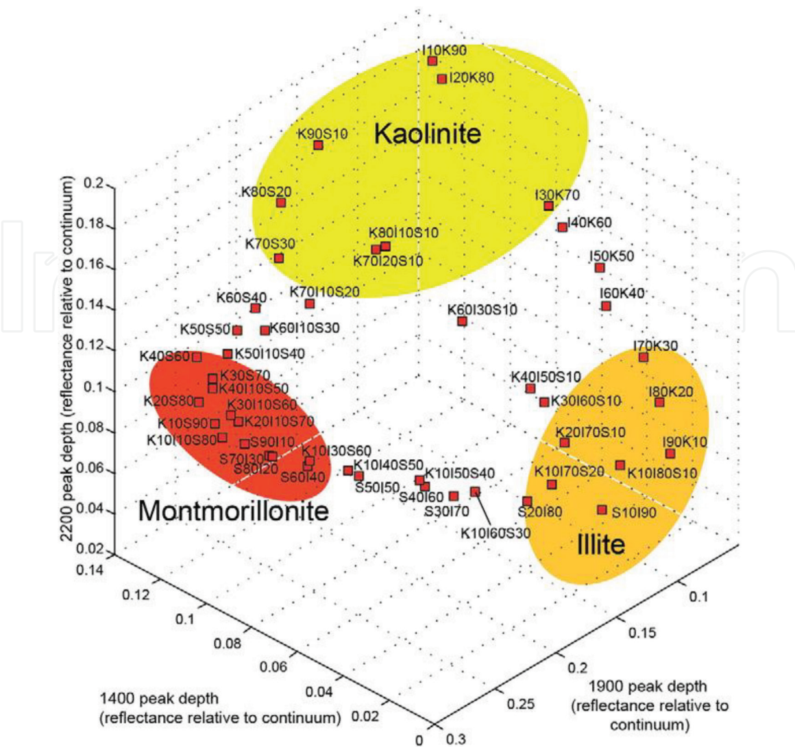
Figure 5. 3D-diagram showing the distribution of the synthetic mixtures according to the depth parameter. From [6].
