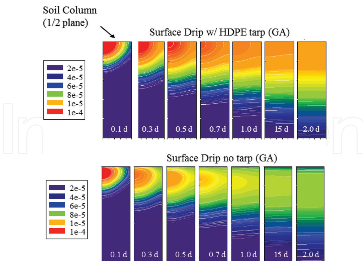
Figure 9. Example use of soil physics model CHAIN_2D where exploration of multiple mitigations strategies such as water sealing, tarps, depth of incorporation, etc. can be simulated, as well as concentration by time ( C \times T ) within soil for biological efficacy.
