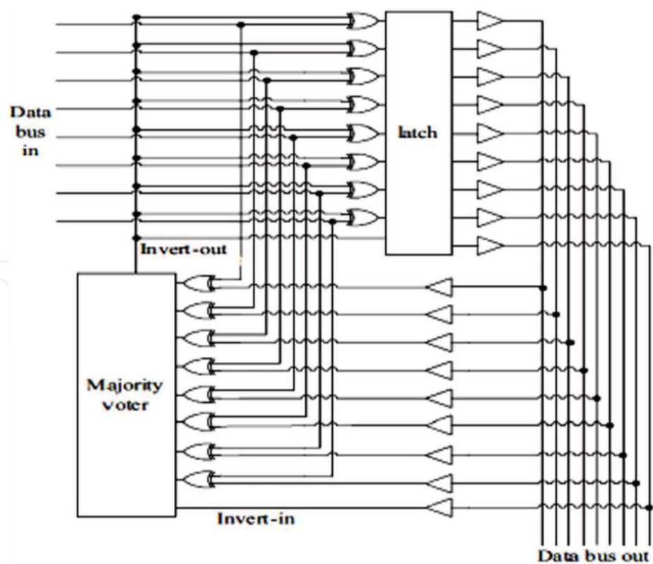
Figure 4. Bus invert method of low-power code.
