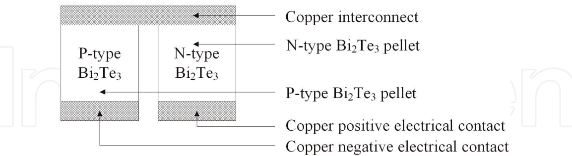
Figure 1. A single thermoelectric couple.
