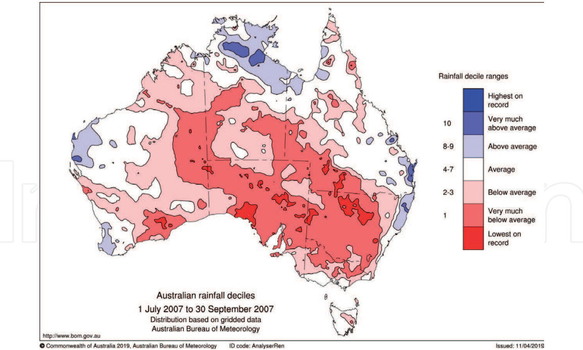
Figure 12. Rainfall deciles for Australia in July–September 2007 derived from the Australian Bureau of Meteorology rain gauge observations.
