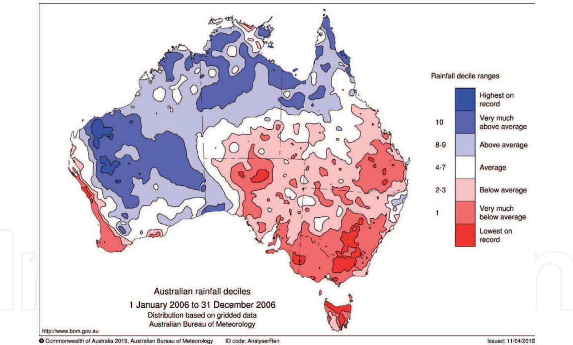
Figure 6. Rainfall deciles for Australia in January–December 2006 derived from the Australian Bureau of Meteorology rain gauge observations.
