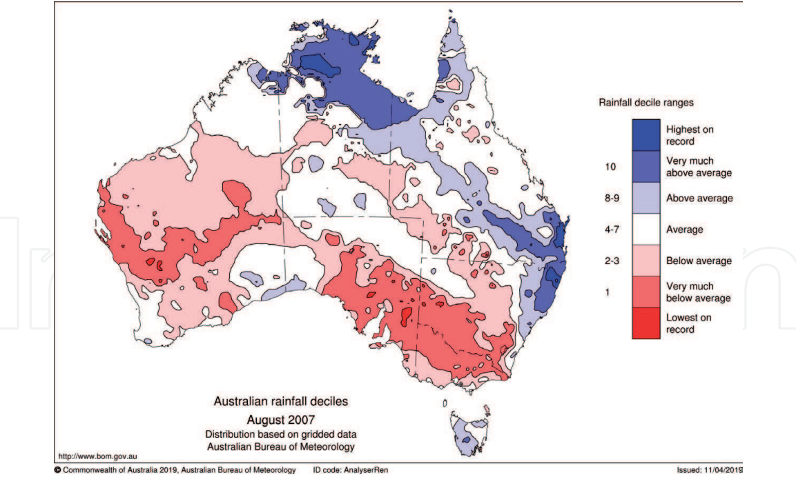
Figure 10. Rainfall deciles for Australia in August 2007 derived from the Australian Bureau of Meteorology rain gauge observations.
