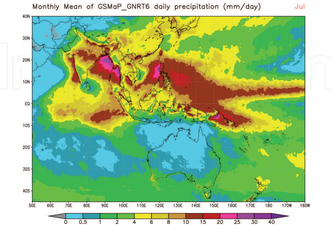
Figure 1. EORC/JAXA GSMaP monthly mean of daily precipitation for the month of July.
