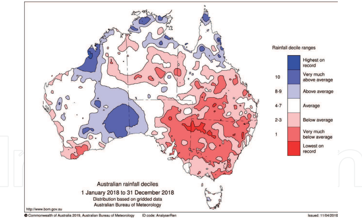
Figure 13. Rainfall deciles for Australia in January–December 2018 derived from the Australian Bureau of Meteorology rain gauge observations.
