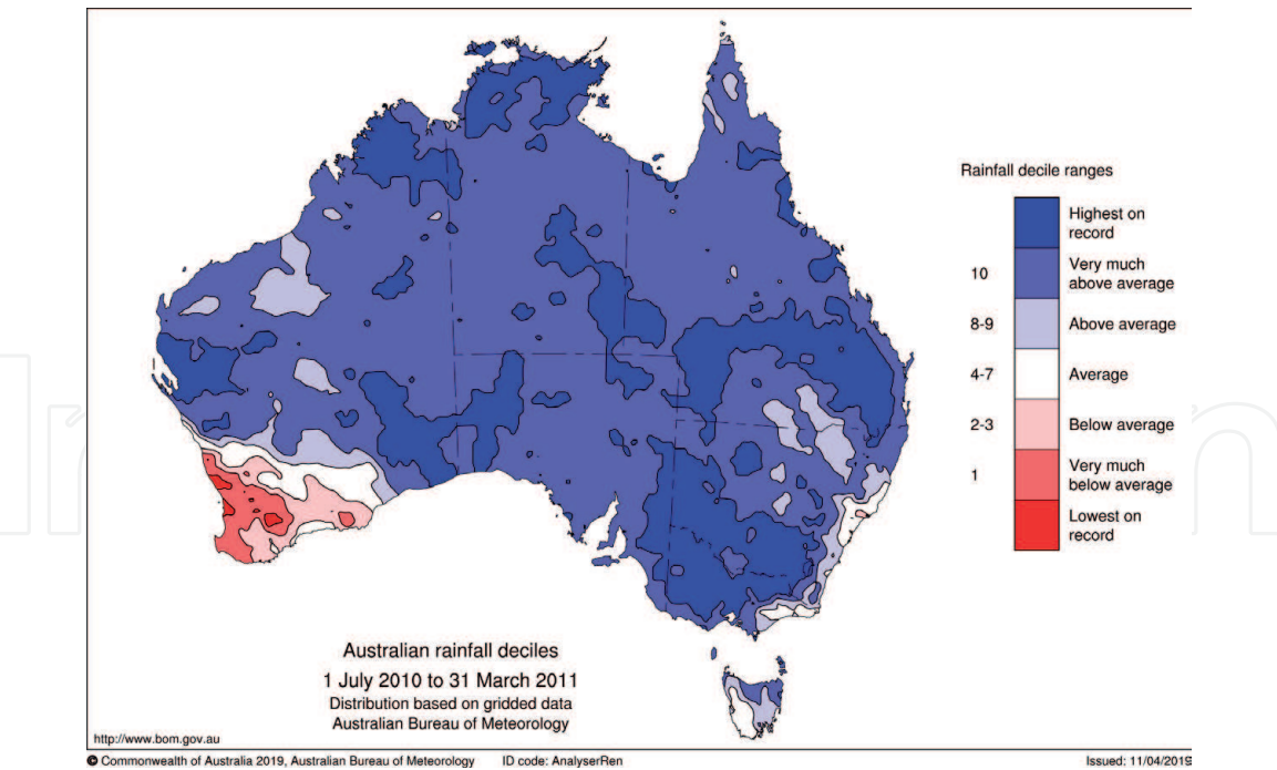
Figure 7. Rainfall deciles for Australia in July 2010–March 2011 derived from the Australian Bureau of Meteorology rain gauge observations.
