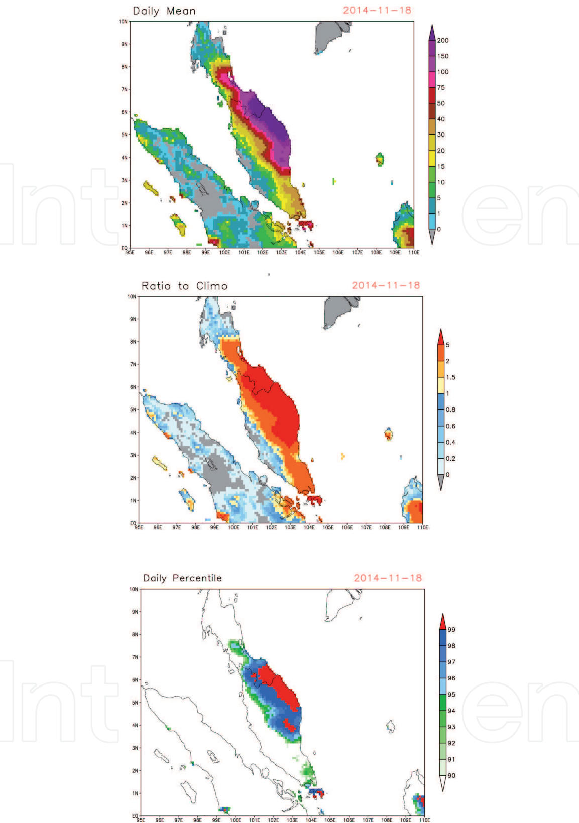
Figure 22. EORC/JAXA GSMaP (a) daily precipitation over the Peninsular Malaysia on 18 November 2014, (b) ratio of the daily precipitation to 18-year climatology, and (c) daily percentile.
