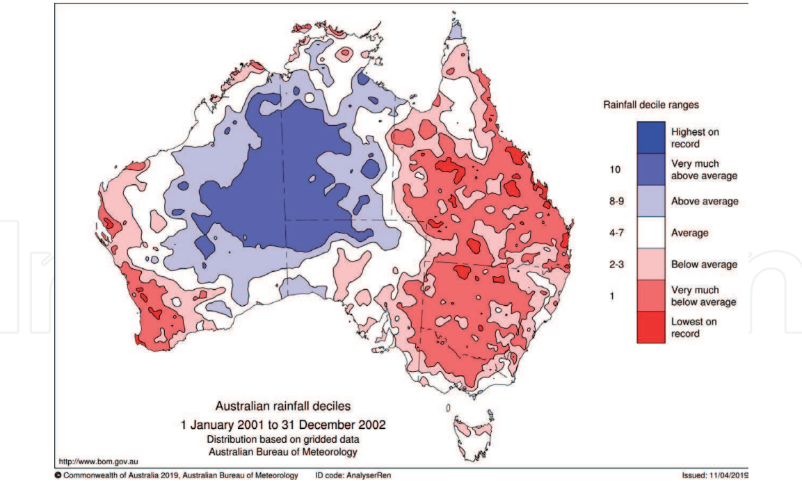
Figure 5. Rainfall deciles for Australia in January 2001–December 2002 derived from the Australian Bureau of Meteorology rain gauge observations.
