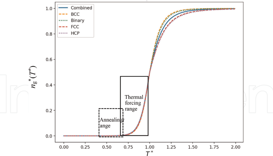
Figure 4. Annealing and thermal forcing regimes of disordered alloys.
