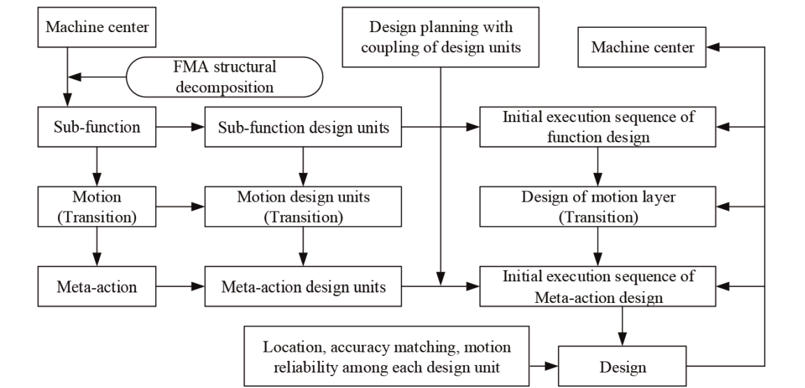
Figure 7. Design process planning driven by FMA structural decomposition.
