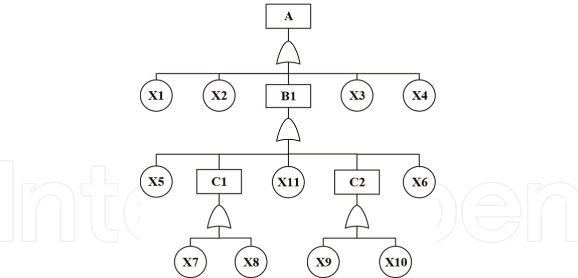
Figure 12. FTA of worm’s vibration.
