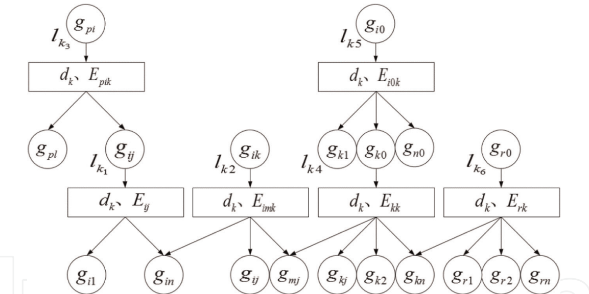
Figure 15. Link network of the assembly error propagation (NBL).
