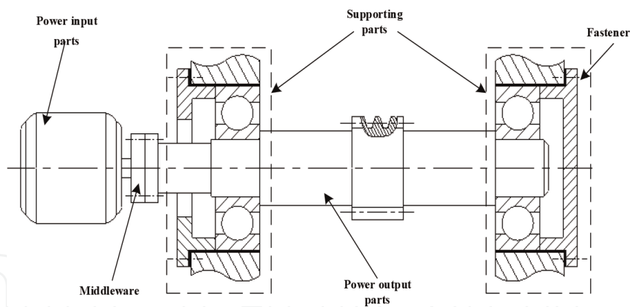
Figure 3. Worm rotating MU.
