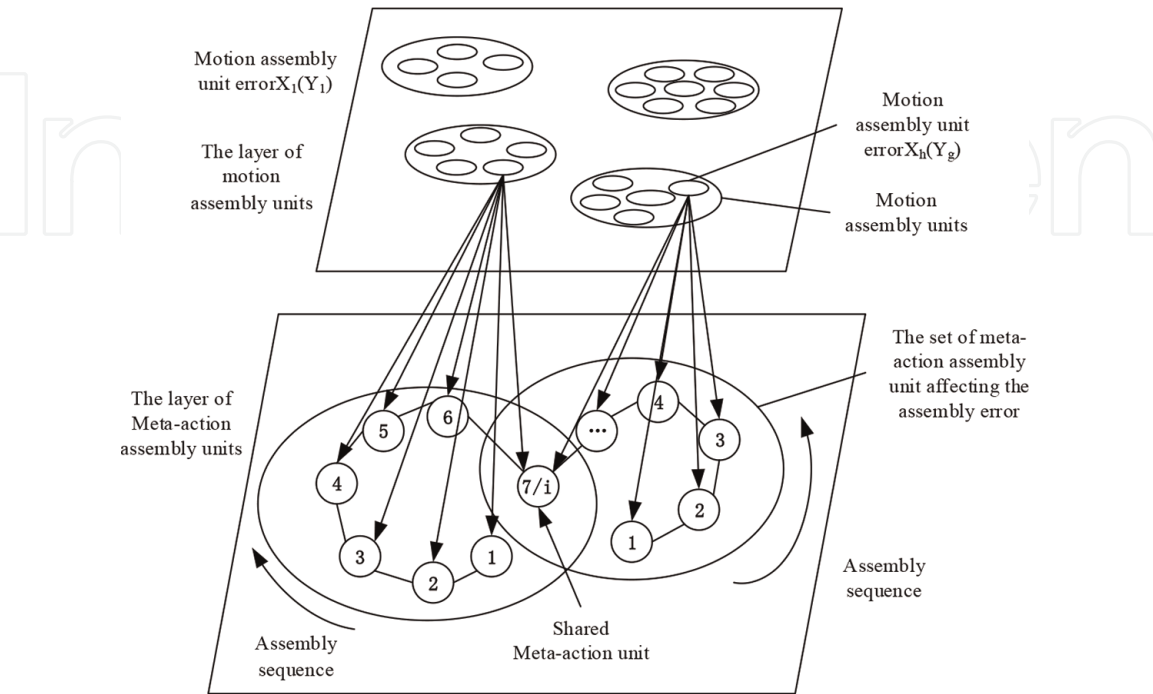
Figure 17. Assembly process from meta-action assembly units to motion assembly units.
