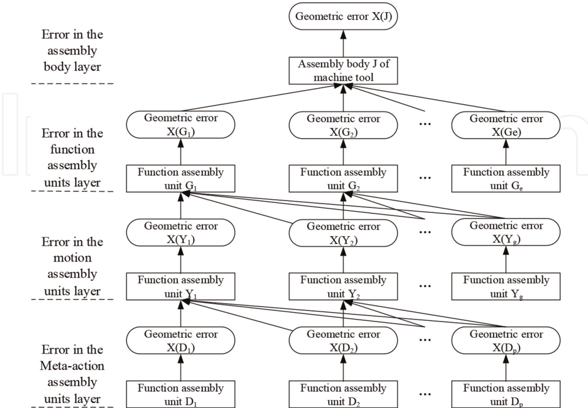
Figure 16. Hierarchy diagram of assembly errors propagation.
