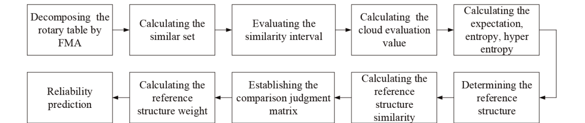
Figure 9. Procedure of reliability prediction based on meta-action units and structure similarity.
