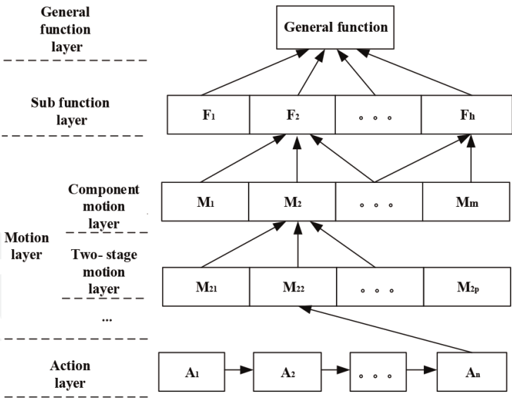
Figure 1. FMA-structured decomposition.
