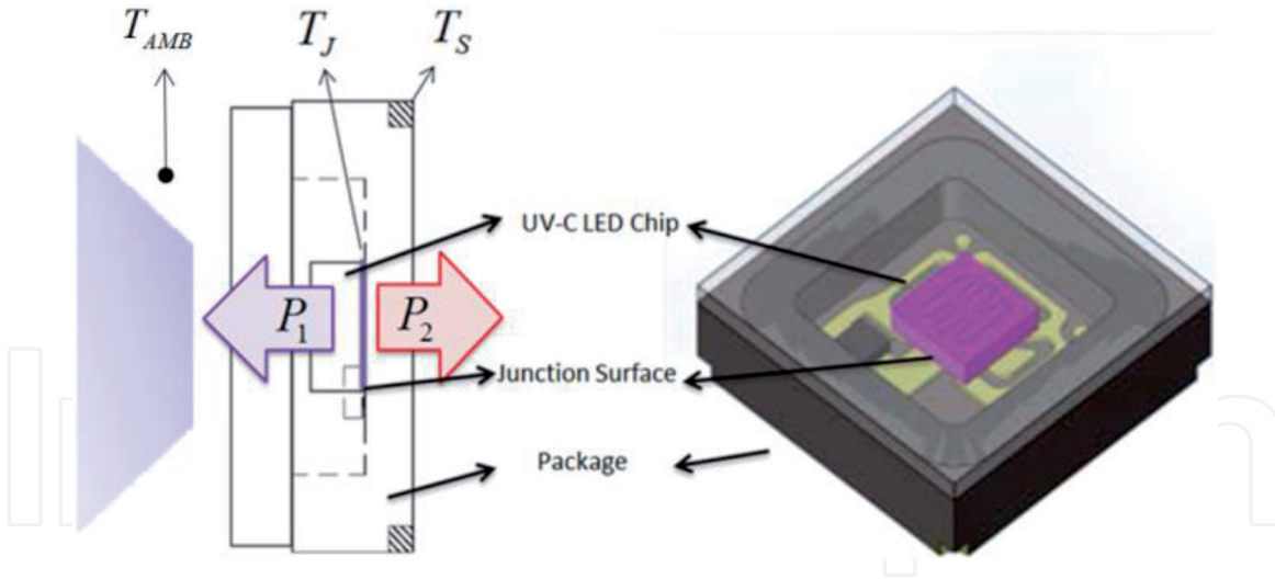
Figure 1. UV-C LED chip inside the package represented in 2D and 3D diagrams. The size of the LED package shown at the right-hand side is 3.6 \times 3.6 mm. T_{AMB} is the ambient temperature, T_J is the junction temperature, and T_S is a solder point temperature.
