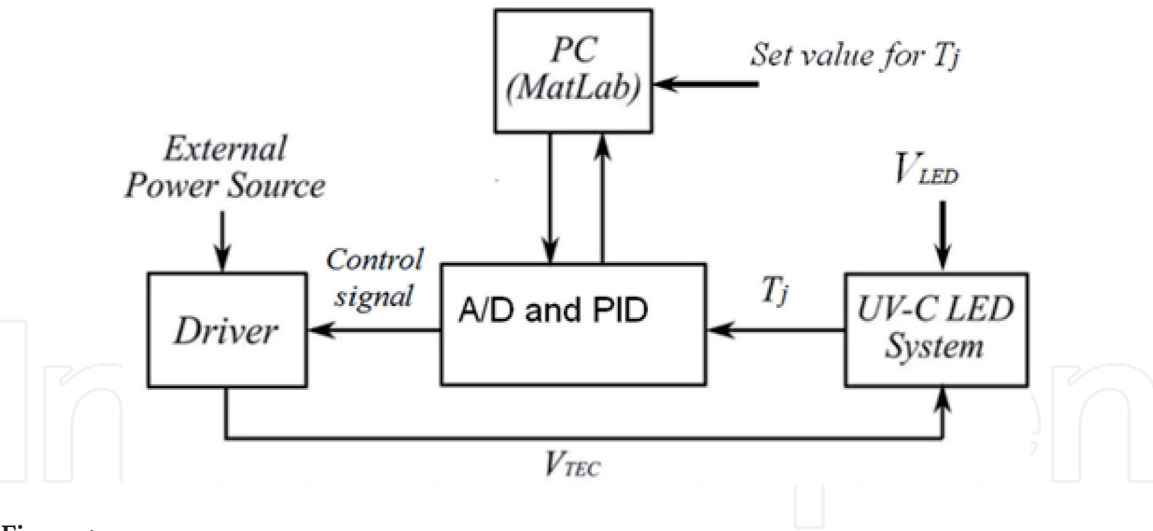
Figure 4. Schematic diagram for the temperature controller.
