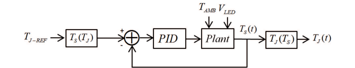
Figure 5. Block diagram for PID controller of T_J based on T_S control.
