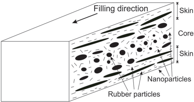
Figure 5. Particle morphology feature scheme.
