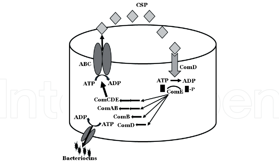
Figure 1. Scheme of the quorum detection system ComCDE and its genes regulated in S. mutans . The ComCDE encodes a signal peptide precursor, which is exported through a specific ABC transporter and generates a competing stimulating peptide (CSP). The ComCDE encodes a component transduction system that specifically detects and responds to CSP. When it reaches a critical concentration CSP interacts with the ComD receptor protein and activates its ComE response regulator. The phosphorylated ComE, in turn, activates the genes downstream, which triggers the signaling cascade for the production of activities dependent on cell density (bacteriocins).
