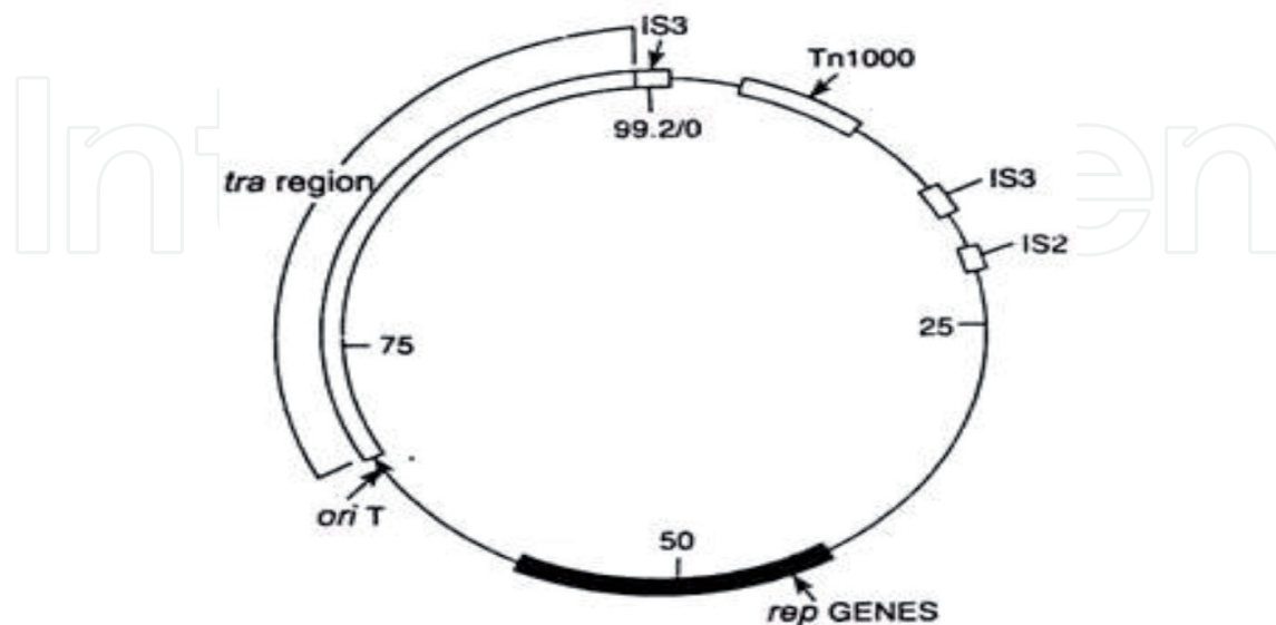
Figure 1. Genetic map of the F-plasmids of E. coli [3].
