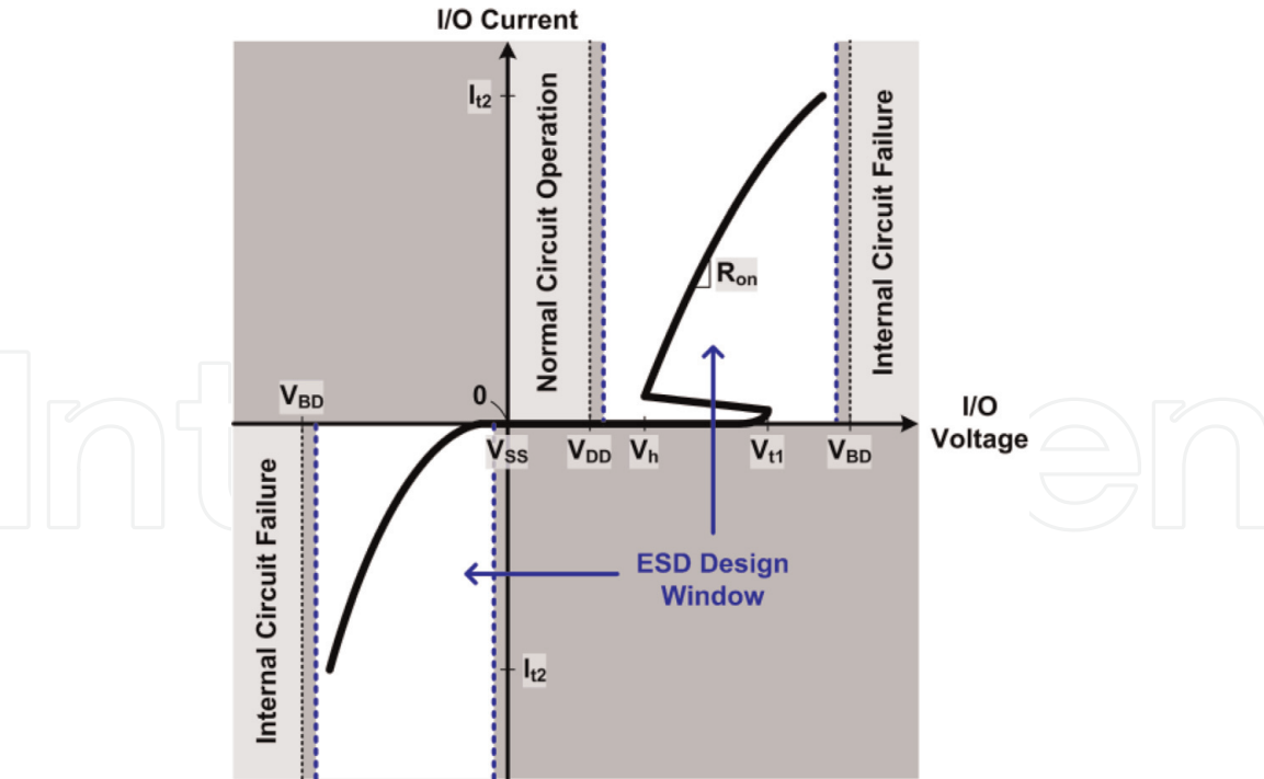
Figure 1. ESD design window.
