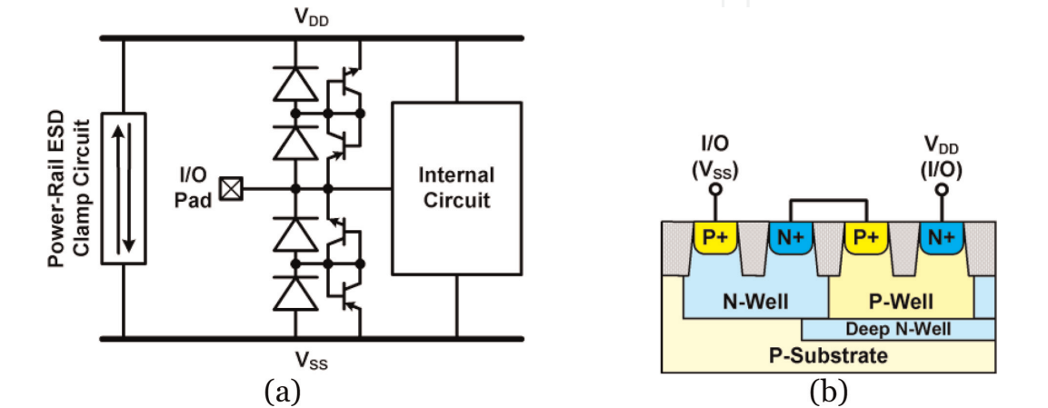
Figure 13. (a) ESD protection circuit with SDSCR and (b) device cross-sectional view of SDSCR.
