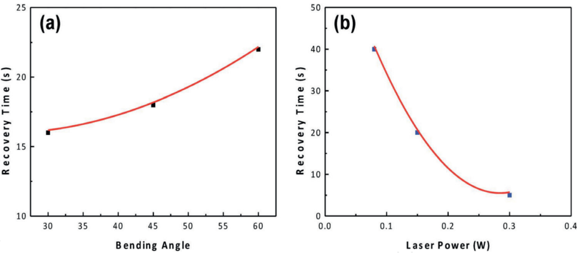
Figure 17. Recovery time versus (a) bending angle and (b) laser power, of the reinforced SMPs with AuNRs at 45° pillar angle [49].
