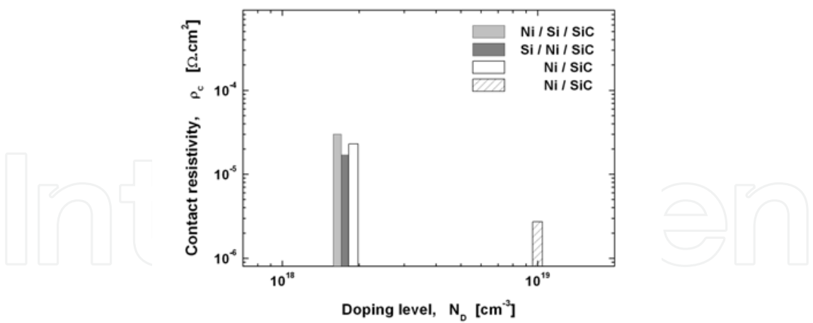
Fig. 2. Dependence of the resistivity of Ni-based contacts to n-type SiC on the substrate doping and the initial contact composition.
