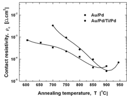
Fig. 9. Dependence of the resistivity of Pd- based contacts on the annealing temperature. obtained after annealing at temperature of 900 °C. This result shows that addition of the refractory titanium into the contact composition shifts the optimal annealing temperature to the higher values. Further increase of the annealing temperature of both contact types causes a resistivity increase. Consequently, the annealing temperature of 850 °C and 900 °C can be accepted as optimal for ohmic properties formation of the Au/Pd and Au/Pd/Ti/Pd contact composition, respectively. The different annealing techniques cause different surface morphology of the Pd-based contacts. The surface morphology of the as-deposited contacts follows the surface features (terraces) of the SiC substrate with a surface roughness of around 1.2 nm and a mean grain size of around 100 nm. After RTA annealing at temperature optimal for both contact types the surface reveals an altered granular structure of the metals. Both grain size and surface roughness are increasing to values of 1-3 μm and 50-100 nm, respectively (Fig. 10 a, b). The annealing in a resistance furnace leads to improved surface morphology and contact properties. The surface roughness (RMS=13 nm) and the mean grain size (150 nm) are smaller (Fig 10 c). However, in this contact structure a strong interdiffusion occurs as can be seen in the AFM image of a scan across the border of a contact pad (Fig. 10 d), where the initial step height between SiC surface and contact pad almost vanishes.
