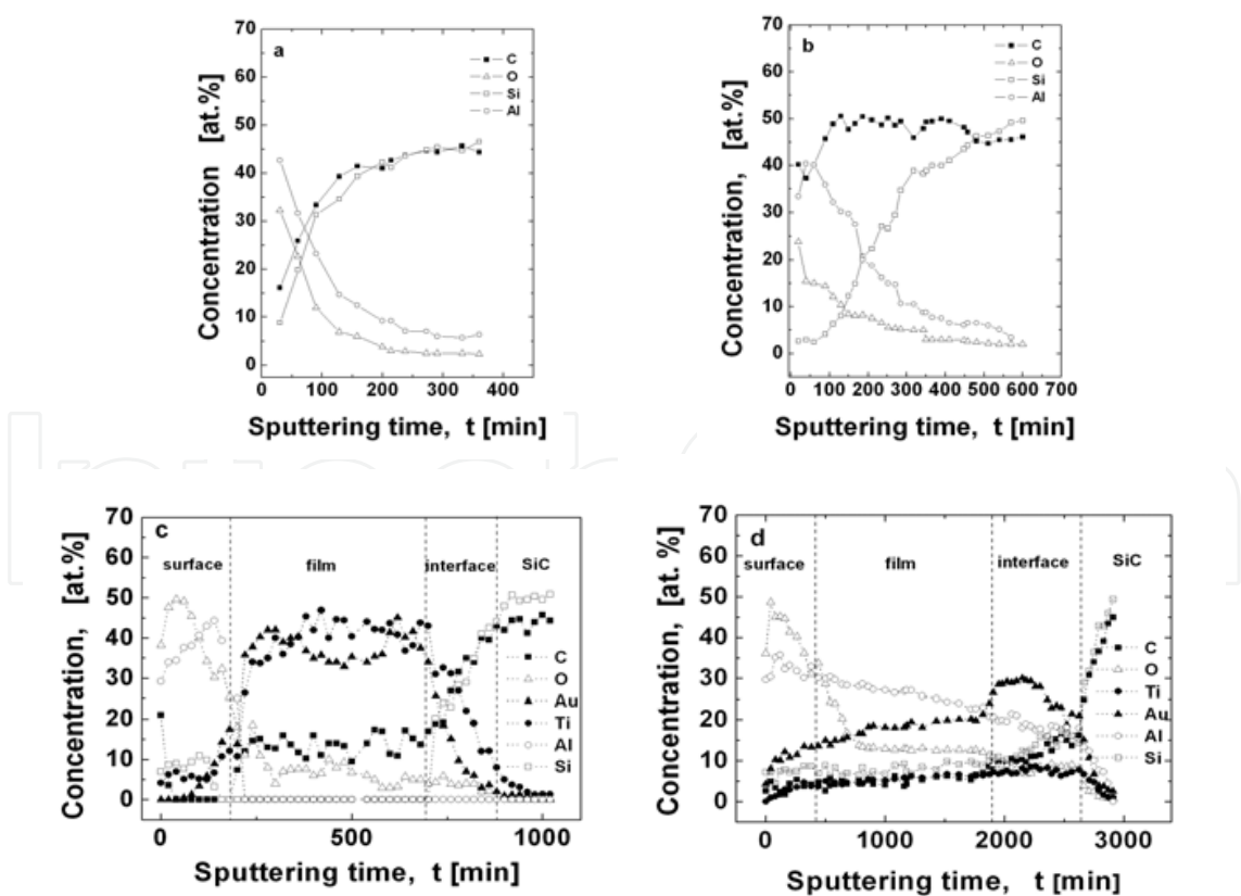
Fig. 8. XPS depth profiles of Al-based contacts: a) Al/Si/SiC; b) AlSiTi/SiC; c) Au/Ti(30%)/Al(70%)/SiC; d) Au/Ti(30%)/Al(70%)/SiC.
