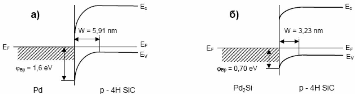
Fig. 20. Energy band diagram of unannealed (a) and annealed (b) Pd/p-type 4H-SiC interface.
