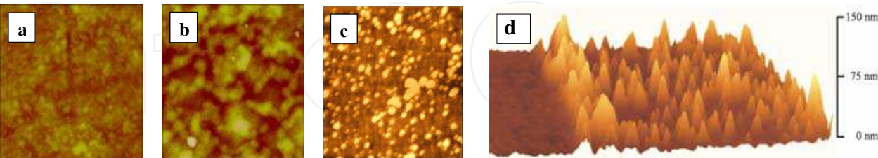
Fig. 10. AFM images: ((25x25) μm², z-scale 1 μm) of RTA annealed Au/Pd/SiC contacts at 850 °C (a) and Au/Pd/Ti/Pd/SiC at 900 °C (b); of RFA annealed Au/Pd/Ti/Pd/SiC contacts at 900 °C - 2D image (5x5 μm², z-scale 50 nm) (c); and 3D image (10x10) μm² across the border between an annealed contact pad and the SiC substrate (d). The XPS depth profile of the as-deposited Pd/SiC and Au/Pd/Ti/Pd/SiC contacts show a steep interface metal/SiC as well as steep interfaces between the metals forming the contact composition (Kassamakova et al., 1999; Kolaklieva et al., 2004). After annealing at an optimal temperature the contact composition changes completely (Fig.11). Annealing of the
