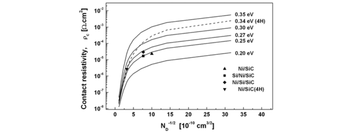
Fig. 3. Comparison of experimentally obtained resistivity values of Ni-based contacts to n-type 6H- and 4H-SiC with theoretical values calculated with different potential barrier heights.
