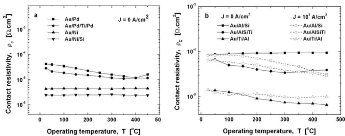
Fig. 13. Dependence of the contact resistivity on the operating temperature and supplied power of: (a) Ni-based and Pd-based contacts, and (b) Al-based contacts Au/Pd/Ti/Pd contacts have demonstrated better stability at operating temperatures in the interval 25 °C – 450 °C in air. For the Au/Pd contacts the contact resistivity decreases twofold as the temperature increased from 25 °C to 450 °C. Similarly, the contact resistivity of the Au/Ti/Al contact decreases with temperature, however at a slow rate. A slow rate decrease is also observed with the Au/AlSiTi contacts from 25 °C to 300 °C. Further
