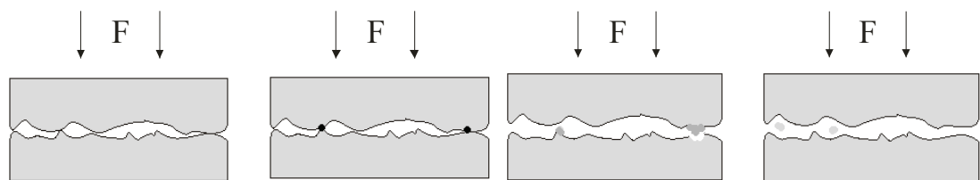
Fig. 3. Illustration of adhesive wear
