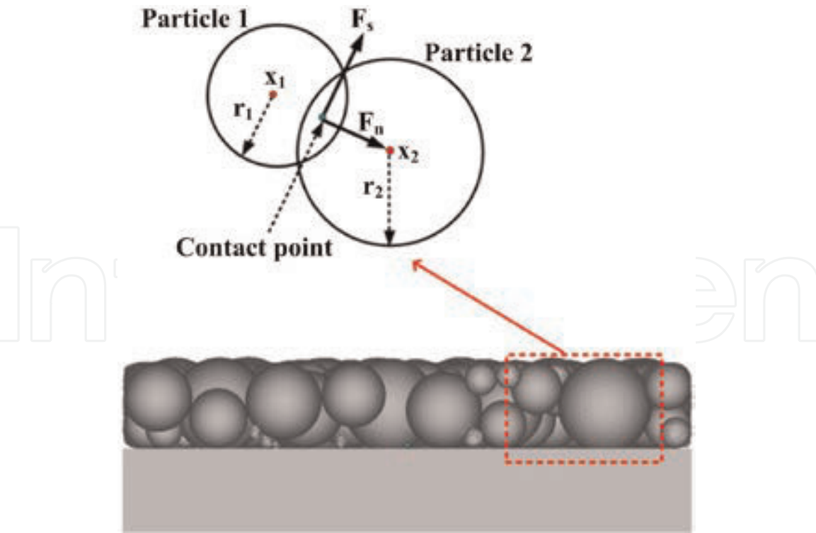
Figure 1. Contact forces generated by interaction between two spherical particles x_1/x_2 and r_1/r_2 are the center and radius of particle 1 and particle 2, respectively.
