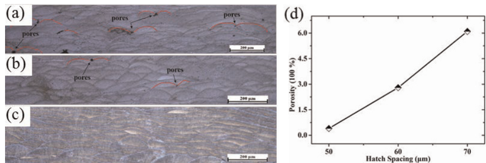
Figure 11. Typical microstructure of the SLM-processed \text{AlSi10Mg} samples at hatch spacing of (a) 70\text{ }\mu\text{m} , (b) 60\text{ }\mu\text{m} , and (c) 50\text{ }\mu\text{m} . (d) Effect of the hatch spacing on the porosity of the as-built sample. The laser power of P = 180\text{ W} , scan speed of v = 1000\text{ mm/s} and layer thickness of d = 35\text{ }\mu\text{m} were fixed in these experiments.
