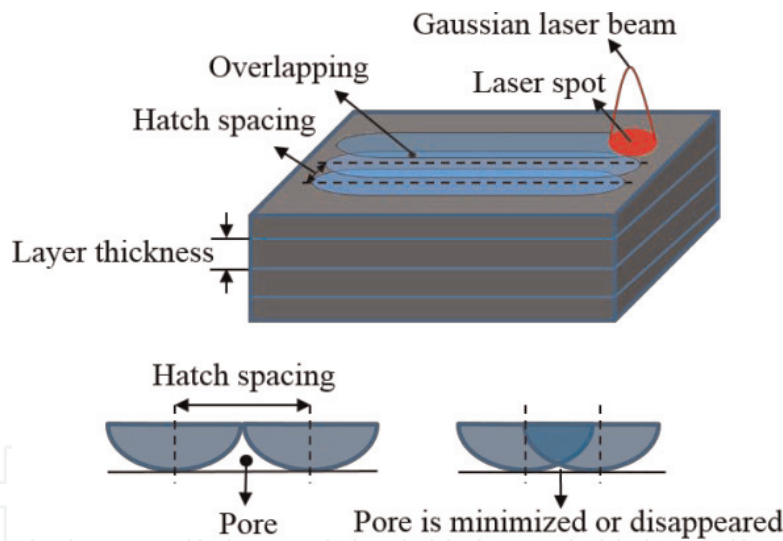
Figure 10. The effect of hatching spacing on the formation of porosity in overlap between adjacent scan tracks.
