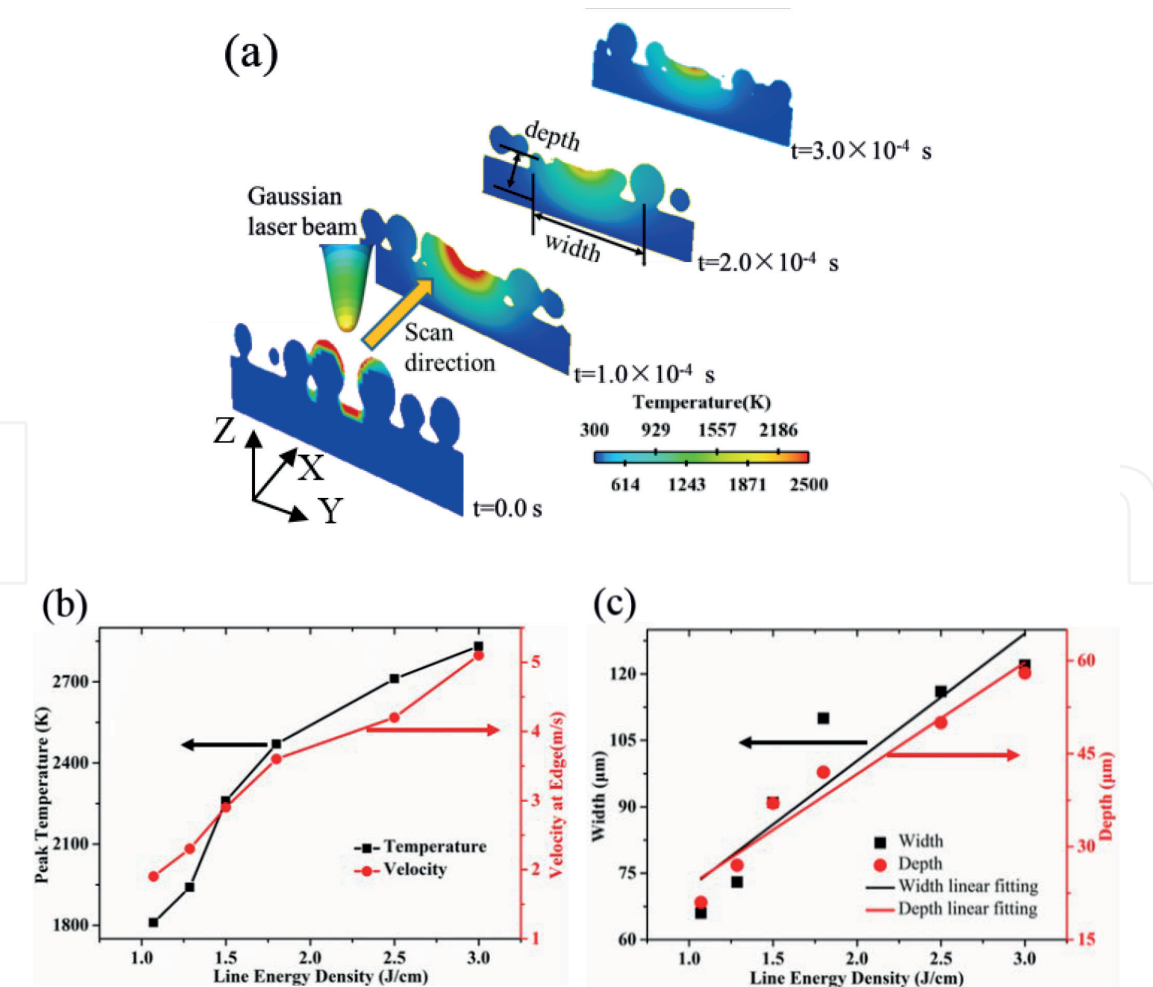
Figure 9. (a) Temperature field and surface melt velocity obtained by simulation at condition of P = 180 W and v = 1000 mm/s. (b) Influence of line energy density on the peak temperature and surface melt velocity of molten pool. (c) Influence of line energy density on the width and depth of molten pool.
