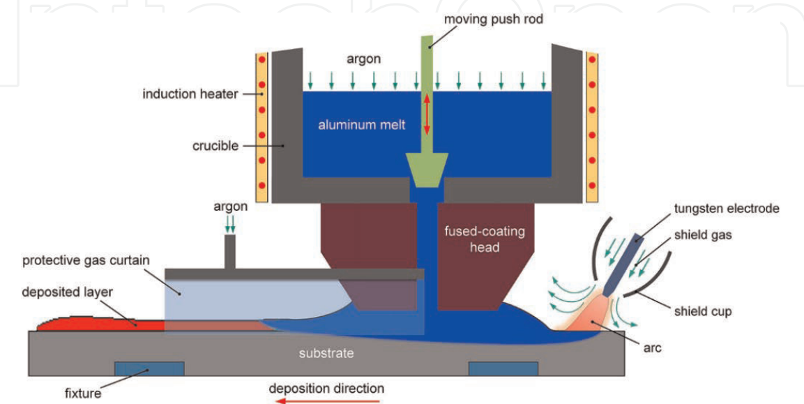
Figure 16. Schematic diagram of MFCAM process.
