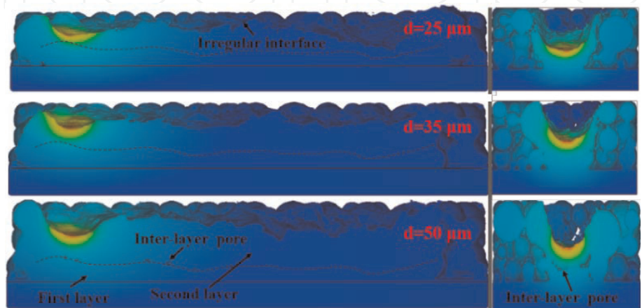
Figure 13. Influence of powder layer thickness on morphology of scan track in longitudinal view (left) and cross-sectional view (right). Laser power P = 180 \text{ W} and scanning speed v = 1000 \text{ mm/s} were fixed in simulations.
