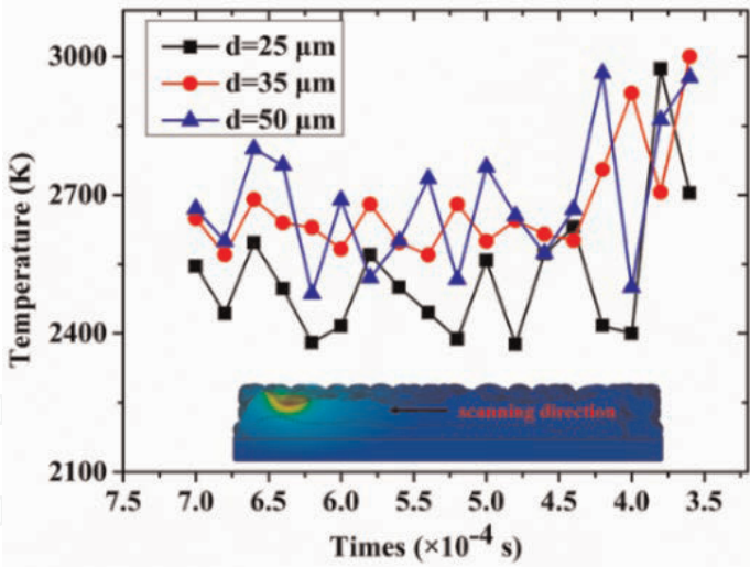
Figure 14. Influence of powder layer thickness on the temperature of molten pool. Laser power P = 180\text{ W} and scanning speed v = 1000\text{ mm/s} were fixed in simulations.
