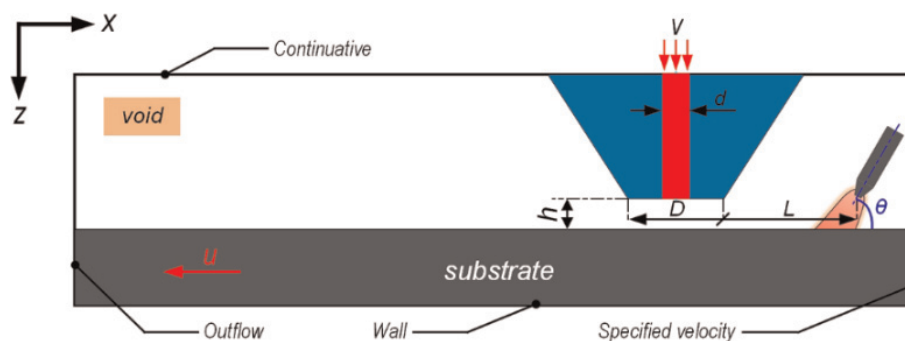
Figure 18. Calculation model for FCAM process.
