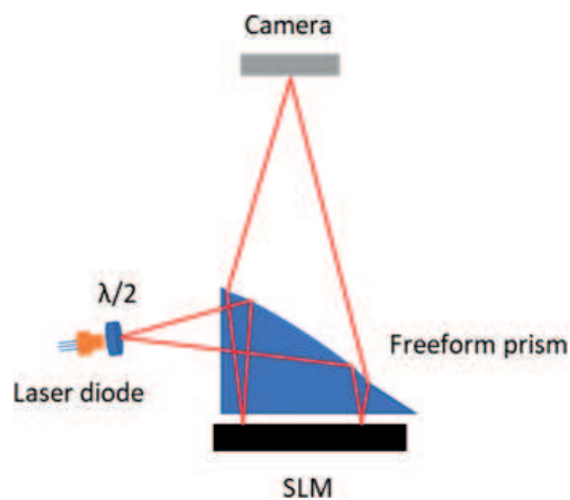
Figure 8. Side illumination of the SLM with freeform prism and the utilization of the total internal reflection [8].
