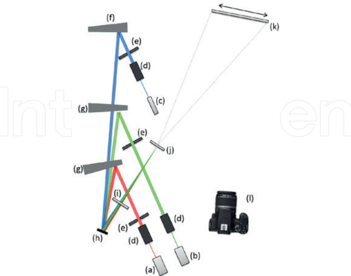
Figure 5. Experimental setup of holographic projection with filtration in the Fourier domain [7].
