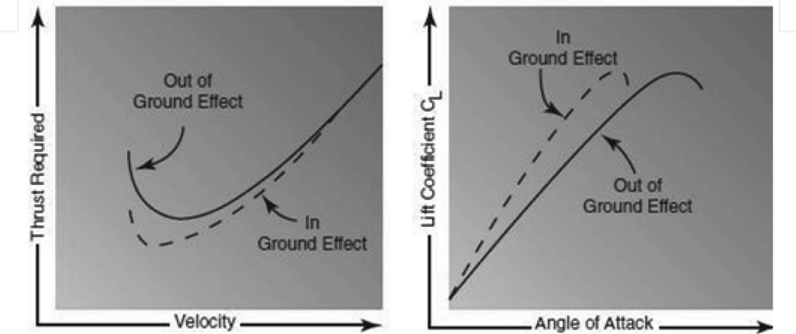
Figure 6. Wing-in-ground effect flight changes drag and lift. Source: Aerodynamics in flight—Airplane ground schools, http://airplanegroundschoools.com/Flight-Aerodynamics/index.html , web source: December 1, 2017.
