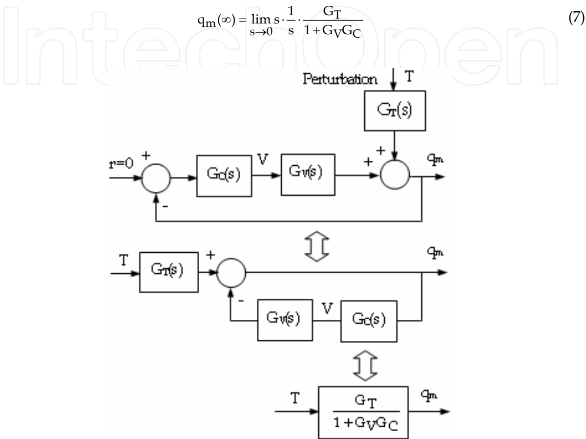
Fig. 12. The equivalent diagram
