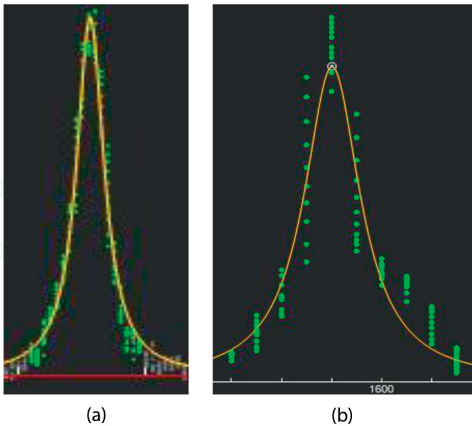
Figure 11. (a) D-band on left (Intensity: 33.5, Center: 1312.4 \text{cm}^{-1} ), (b) G-band on right (Intensity: 62.5, Center: 1580.2 \text{cm}^{-1} ) for graphene nanoplatelets (ammonia) with 780 nm excitation and using fityk peak fitting software [14].
