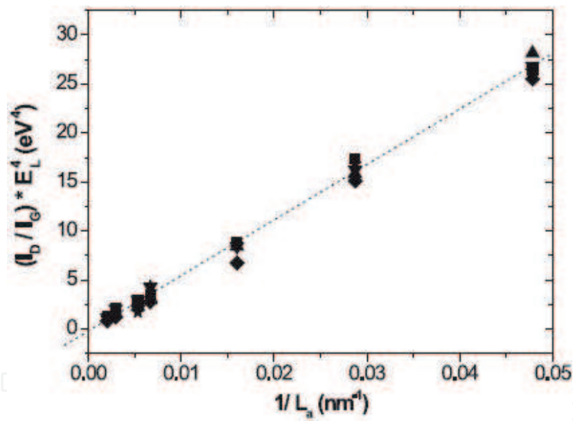
Figure 9. Plot of (I_D/I_G) \cdot E_L^4 vs. 1/L_a . E_L is the laser excitation energy in eV, I_D and I_G are the D and G band intensities, respectively, and L_a is the characteristic lateral size of the graphene layer. Adapted from [5].
