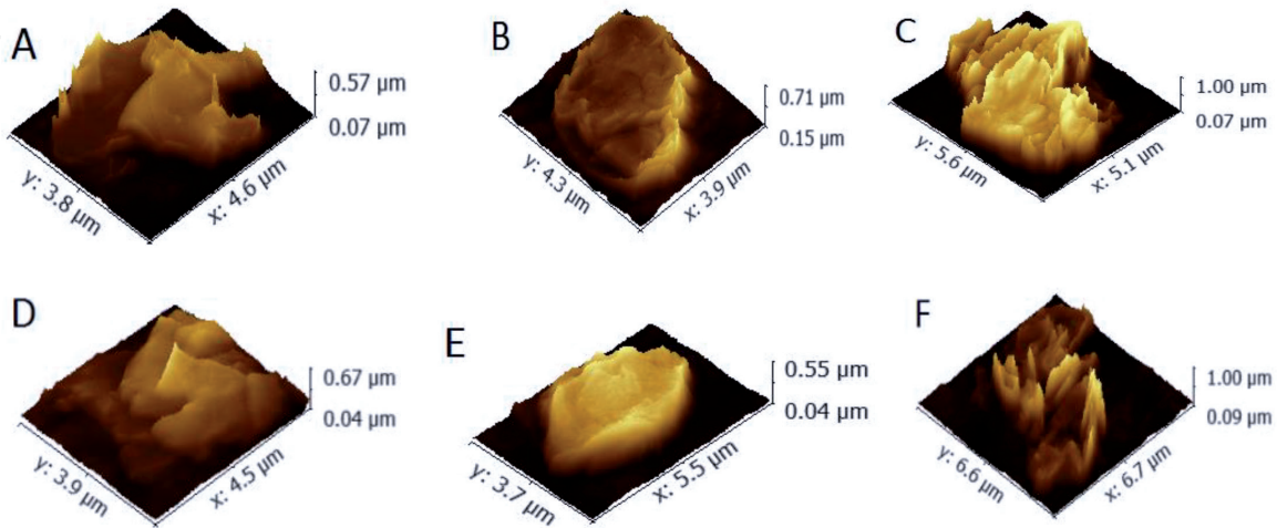
Figure 10. 3D view of SEM data of functionalized graphene nanoplatelet aggregates doped with argon (A), carboxyl (B), oxygen (C), ammonia (D), fluorocarbon (E), and nitrogen (F), respectively, using Gwyddion software.
