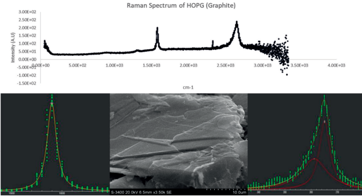
Figure 8. (Top) Raman spectrum of HOPG graphite at excitation of 780 nm. (Bottom left) G-band and Lorentzian ( 1579.7\text{ cm}^{-1} , height: 128.9); (Bottom middle) SEM image of HOPG sample; (Bottom right) G'-band and Lorentzians ( 2611.8\text{ cm}^{-1} , 2651\text{ cm}^{-1} , heights: 56.1, 123.1).
