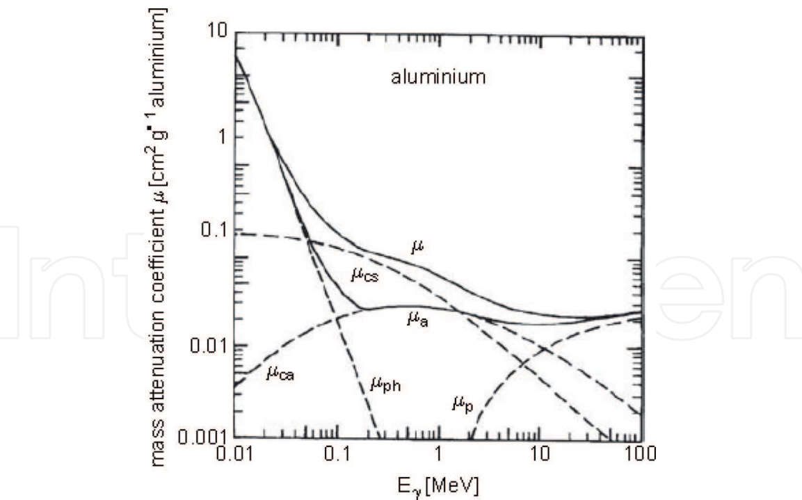
Figure 8. Energy dependence of the mass attenuation coefficient \mu and mass absorption coefficient \mu_a for photons in Aluminum.
