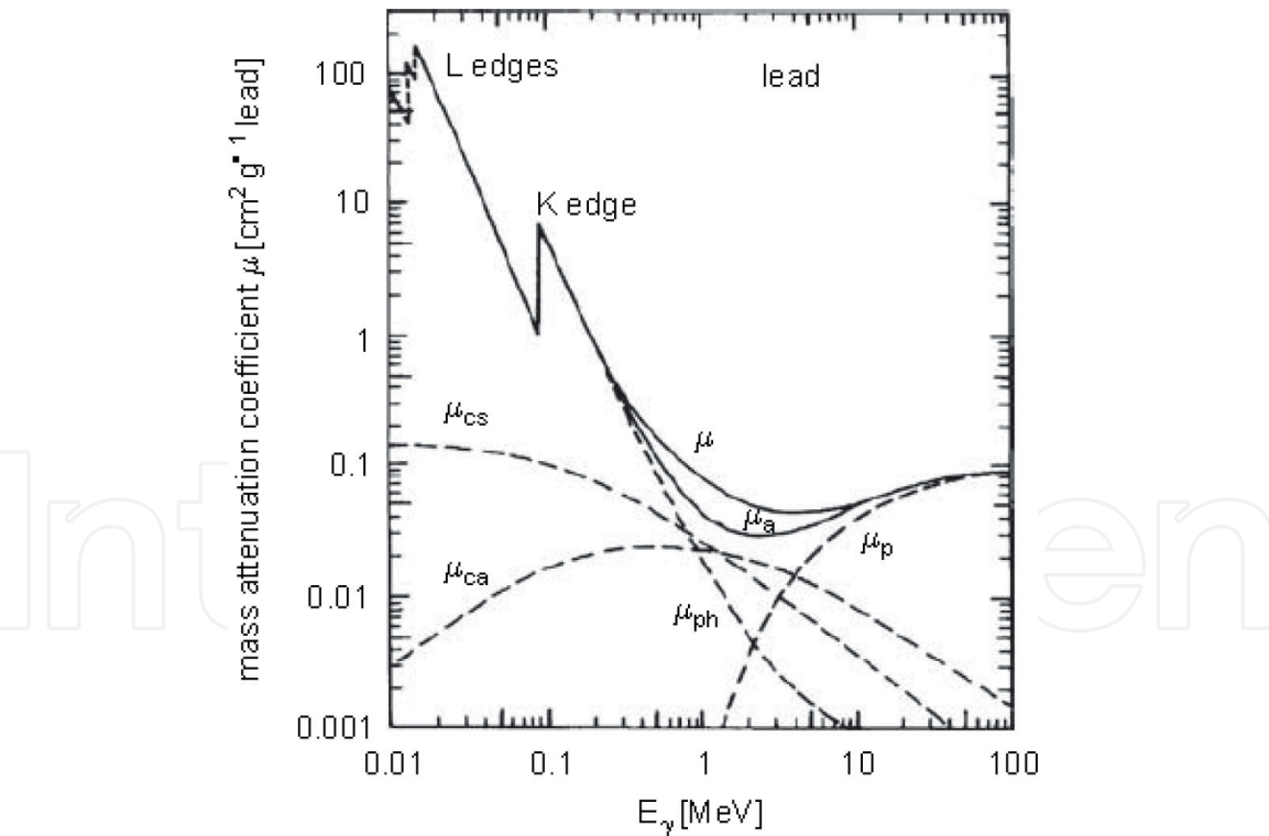
Figure 9. Energy dependence of the mass attenuation coefficient \mu and mass absorption coefficient \mu_a for photons in Lead.
