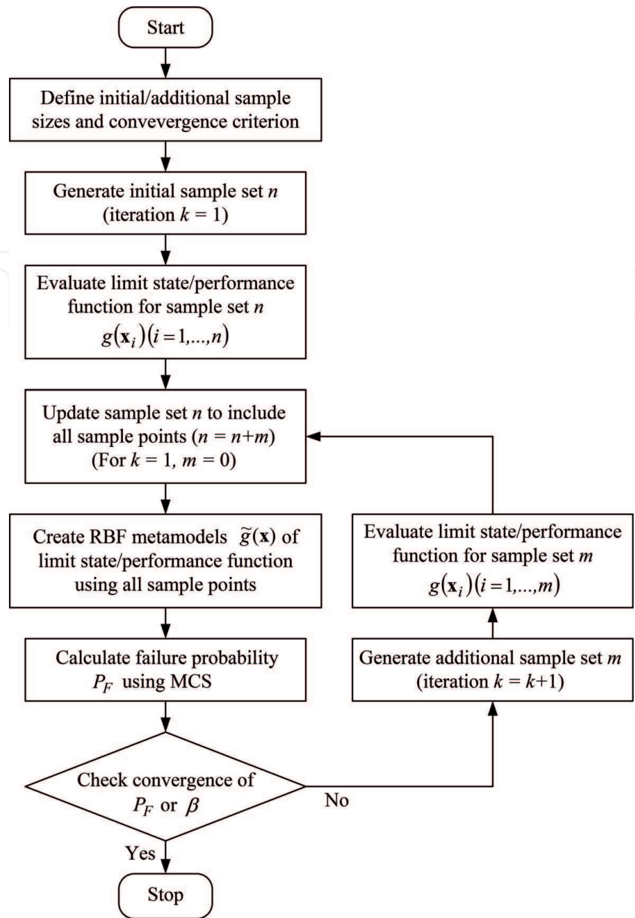
Figure 1. Flowchart of reliability analysis using a SRBF surrogate technique.
