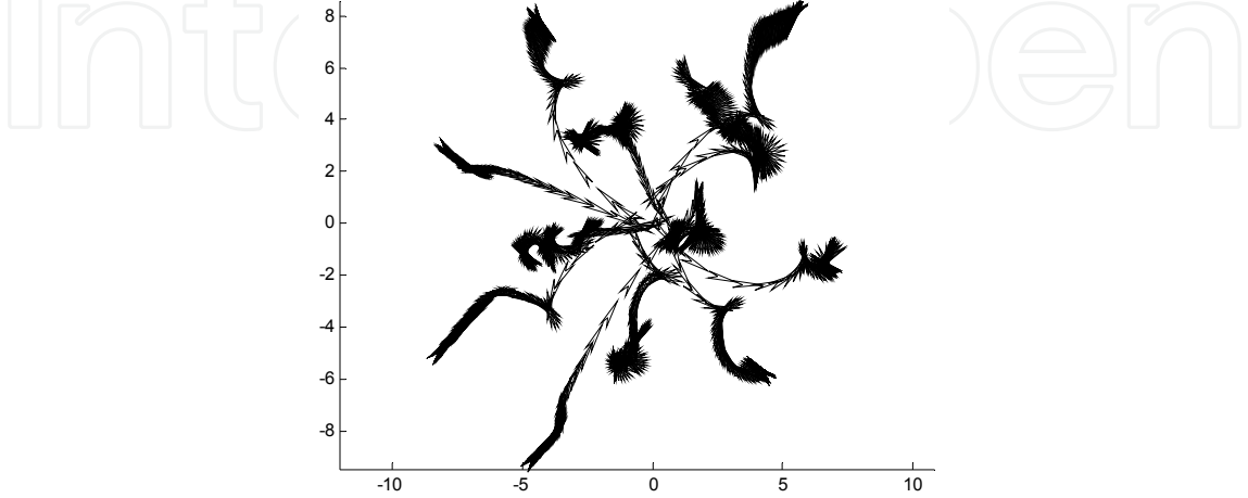
Fig. 7. Deployment paths for 12 nonholonomic mobile robots
