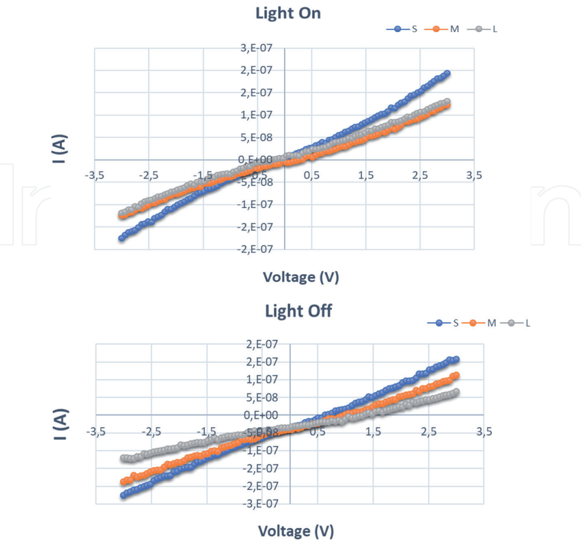
Figure 16. Top: I-V curves measured in the presence of white light and using four-point method MoS 2 film. Bottom: I-V curves measured film in dark-room under otherwise conditions. When comparing both measurements it is possible to observe a change on slope, which is related to resistive values as presented in Figure 17.
