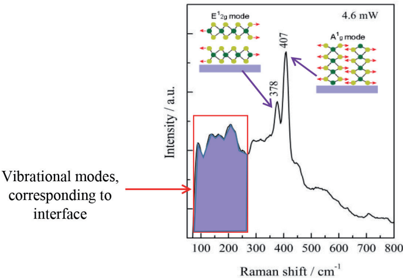
Figure 10. The Raman spectra with two characteristic modes of vibrations at E 2g at 378 cm -1 and A 1g at 407 cm -1 , in agreement with Kong et al. [19].
