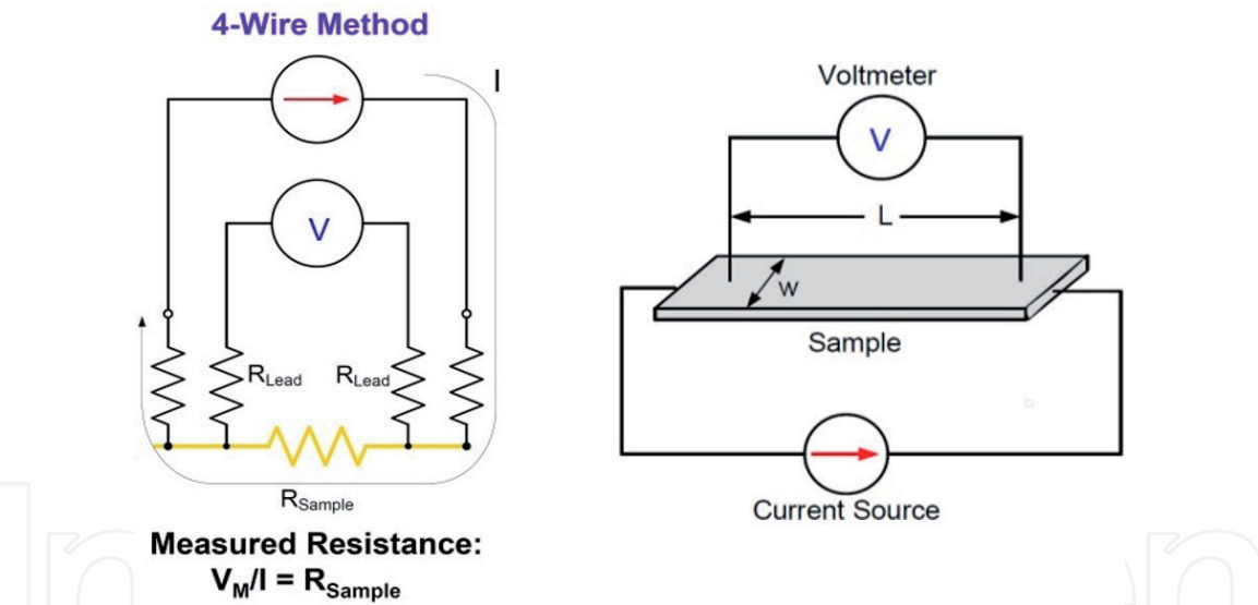
Figure 15. Graphical description of the four-point method implemented for electrical transport in MoS 2 film.
