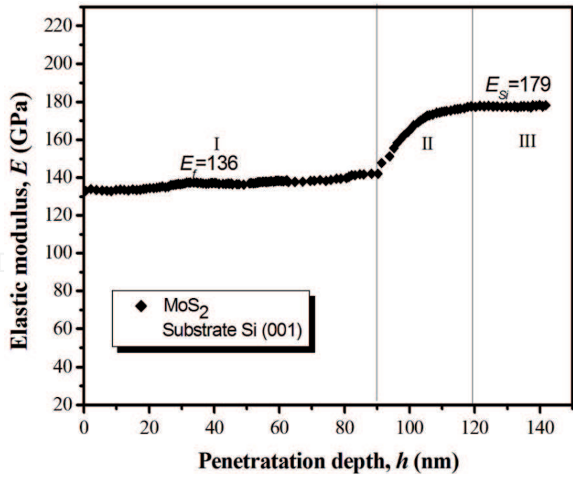
Figure 12. Nanoindentation curves estimated experimentally using continuous stiffness method (CSM), the curve corresponds to regions I, II, III. In region I the estimated elastic modulus is E = 136 \pm 2 GPa corresponds to 0–90 nm of penetration depth, which is indicated to be only for MoS 2 film, in agreement with [28].
