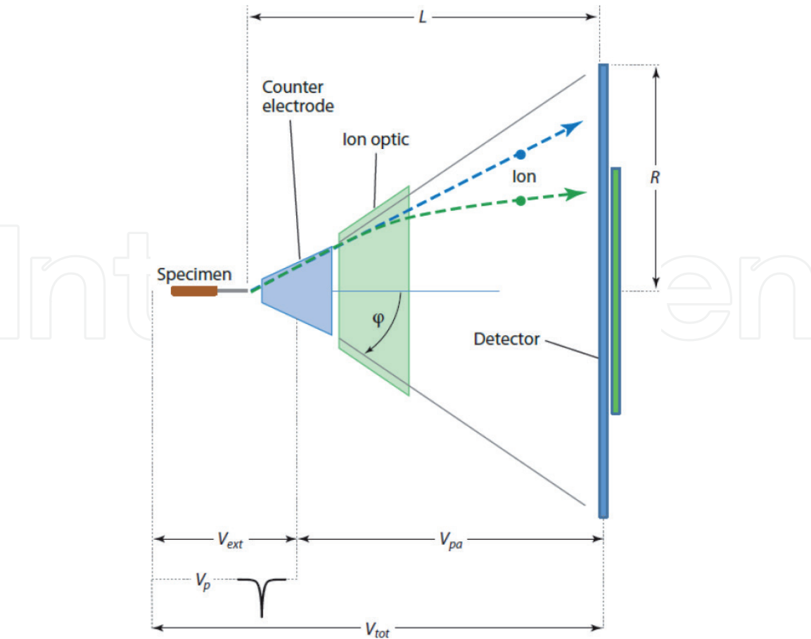
Figure 6. Schematic drawing of APT (taken from [23]).
