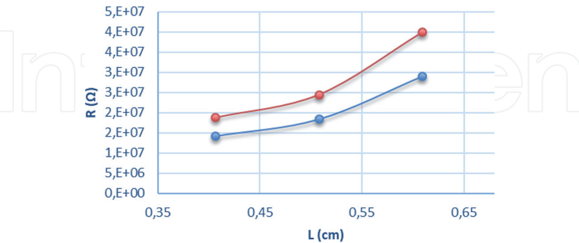
Figure 17. Resistivity \rho values, calculated from I-V curves measured in the presence of white light and dark environment by using four-point method over MoS 2 film's surface. Red curve corresponds to presence of light shining on surface and blue curve to dark-room conditions.
