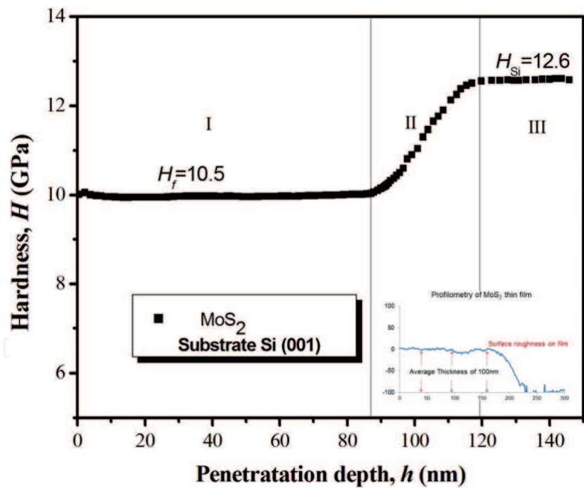
Figure 13. The region I corresponds to hardness values of H = 10.5 \pm 0.1 GPa at 0–90 nm of penetration depth corresponding to MoS 2 layer. The regions II and III on both curves corresponds to mixed stage MoS 2 /SiO 2 and SiO 2 substrate reason of an increase on both values are observed, in agreement with [28].
