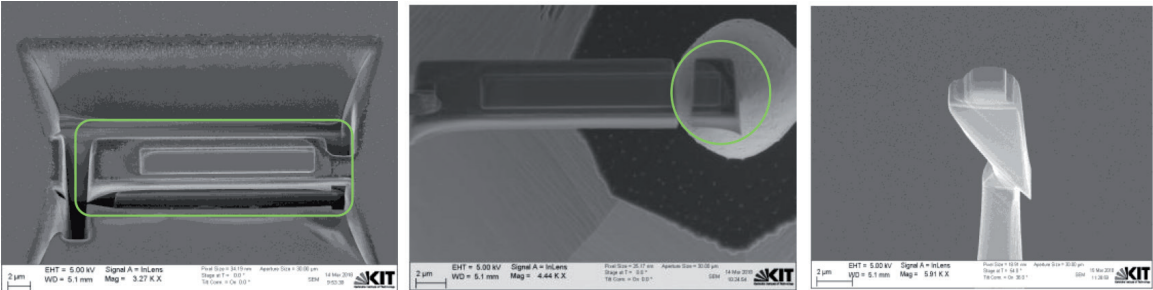
Figure 7. Scanning electron images taken during lift-out procedure to prepare a needle for atom probe tomography in MoS 2 thin film (green square and circles are the areas of interest and cut using Ga ions and Omiprobe® micromanipulators), as discussed by Szász et al. [21].
