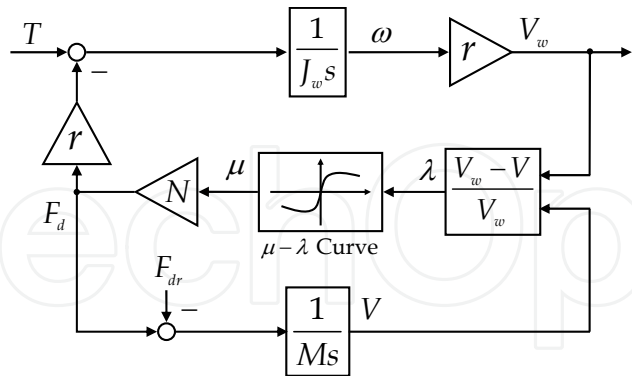
Fig. 2. One-wheel vehicle model with Magic Formula.
