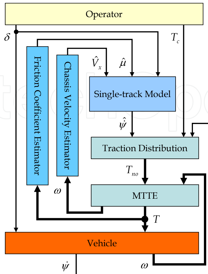
Fig. 15. A DYC system based on MTTE
