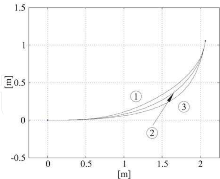
Fig. 7. Modifying a clothoid by perturbing \dot{\kappa}_B .
