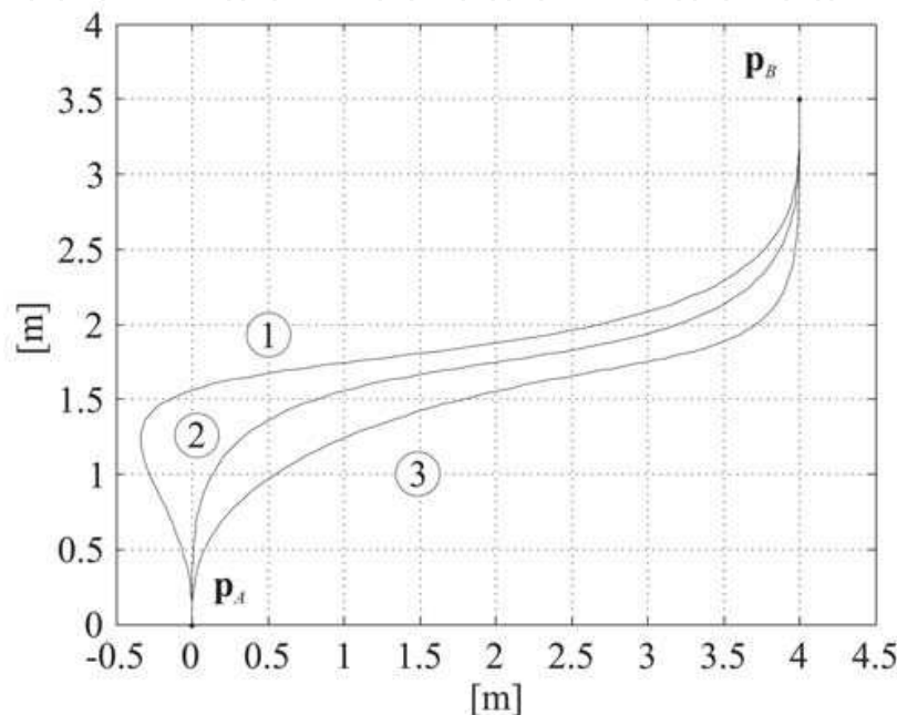
Fig. 6. Modifying a lane-change curve by perturbing \dot{\kappa}_A .
