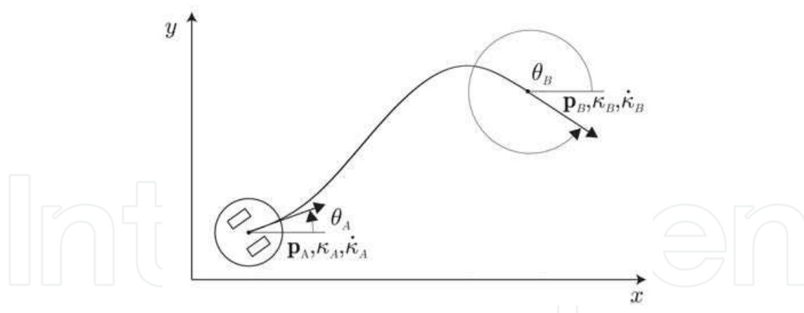
Fig. 1. A G^3 -path connecting \mathbf{p}_A with \mathbf{p}_B for the SMPP.
