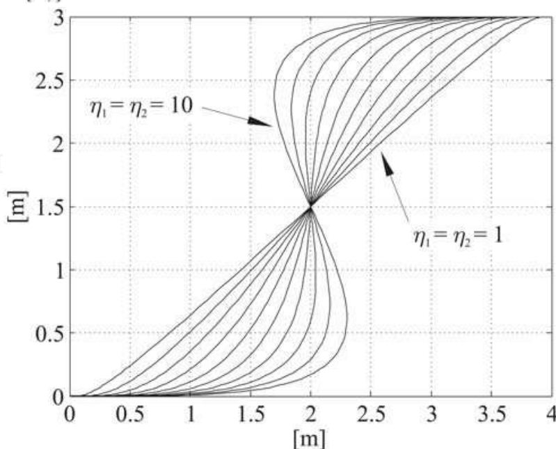
Fig. 3. Lane-change curves with \eta_3 = \eta_4 = \eta_5 = \eta_6 = 0 .
