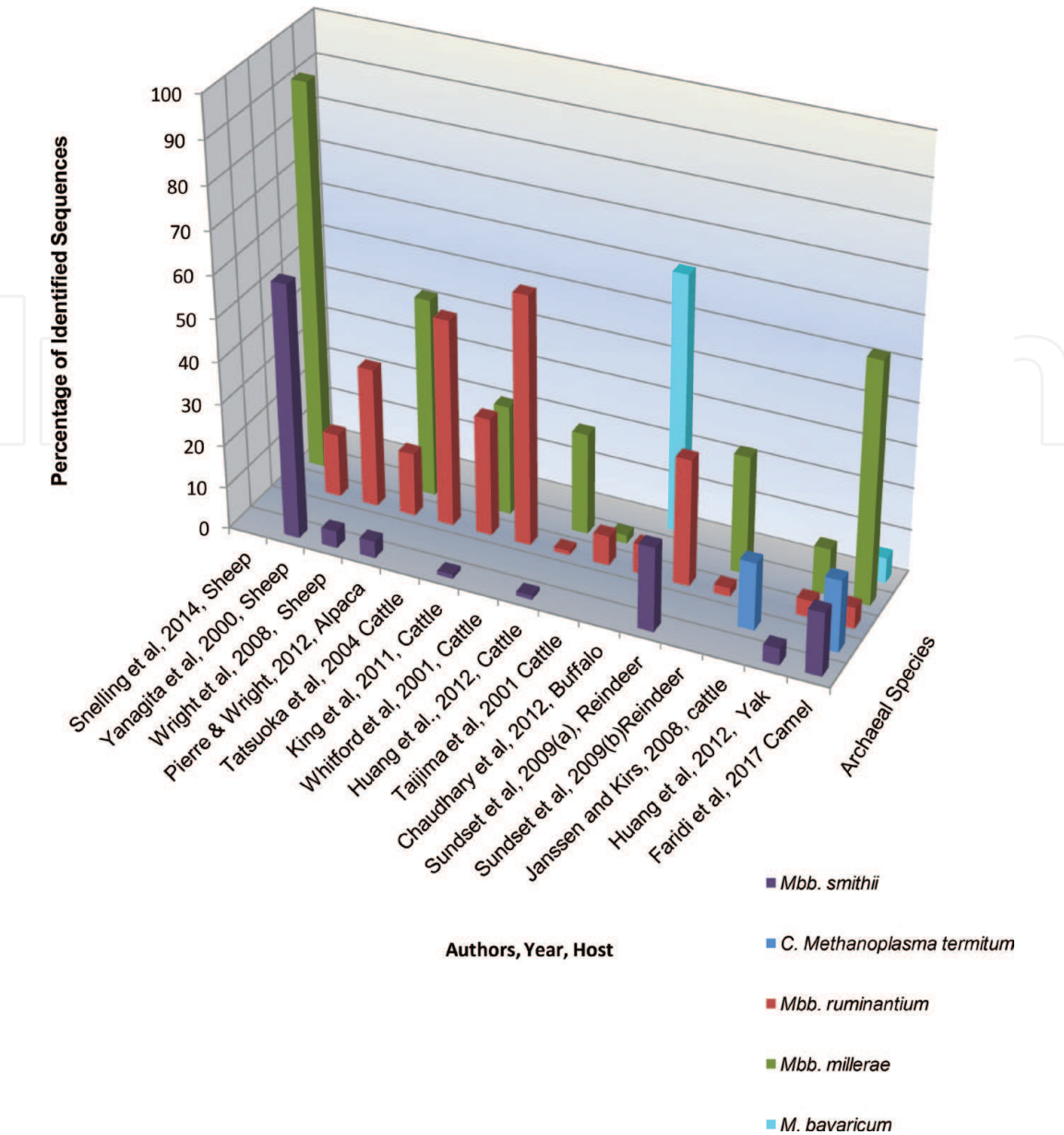
Figure 2. Methanogenic sequences identified in ruminants around the world.
