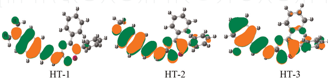
Figure 2. HOMO orbitals of triazine-based hydrazone derivatives.
