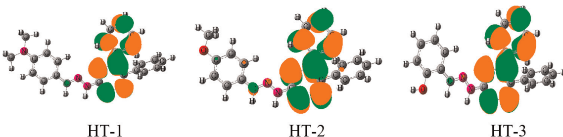
Figure 3. LUMO orbitals of triazine-based hydrazone derivatives.
