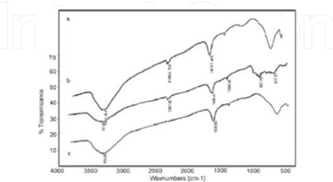
Figure 8. Infrared spectra of \text{LaCrO}_3 calcined at (a) 600°C, (b) 700°C, and (c) 800°C [48].
