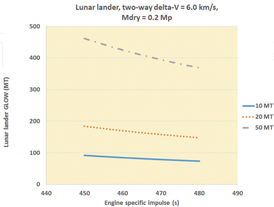
Figure 14. Lunar lander masses versus specific impulse: 6 km/s delta-V capability.
