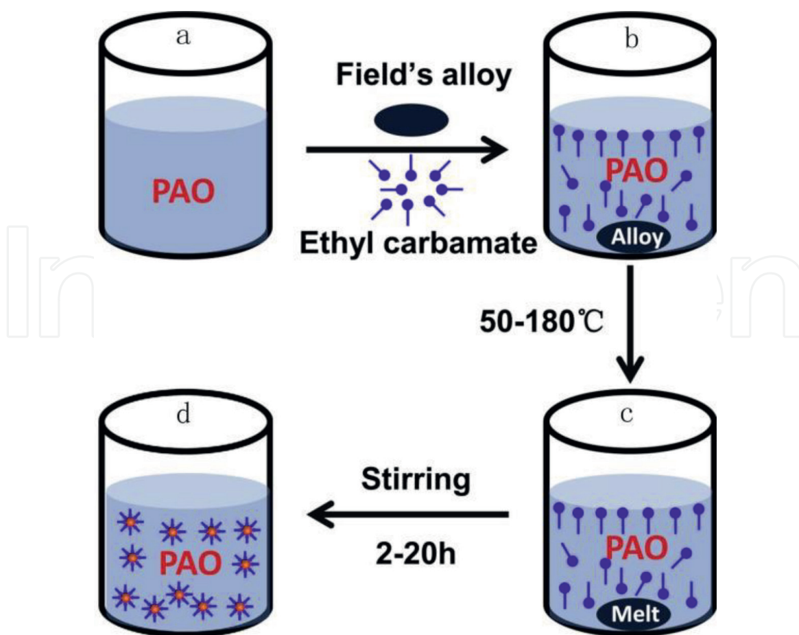
Figure 1. Illustrated scheme of the synthesis of molten Field's alloy nanoparticles using nanoemulsification method. (a) PAO and molten Field's alloys are in the reaction vessel. These two liquids are immiscible and phase separate; (b) polymer surfactant (ethyl carbamate) is soluble in PAO; (c) the mixture is heated up to certain temperature and the bulk molten alloy formed; (d) the microscale emulsion is stirred and breaks into microscale droplets until nanoemulsion is formed.
