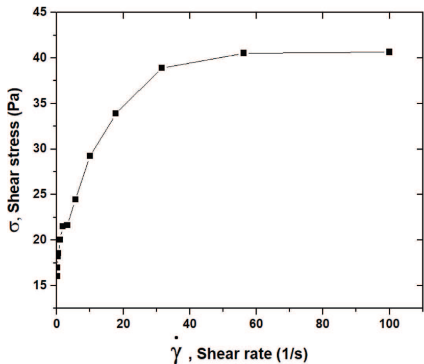
Figure 16. Yield test for an NRGF fuel.
